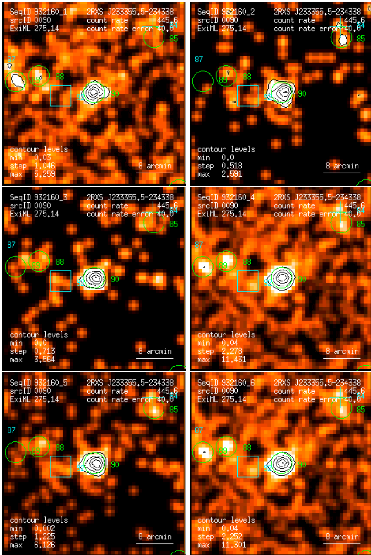
Figure 90: RASS 932160: detection 0090: band rate images, Gaussian filter: (1) PSPC channels 11 – 41, (2) 52 – 90, (3) 91 – 201, (4) 11 – 235, (5) 52 – 201, (6) 11 – 201. Broad band rates in counts/ks. Band rate contour levels in counts/ks/arcmin 2 .
