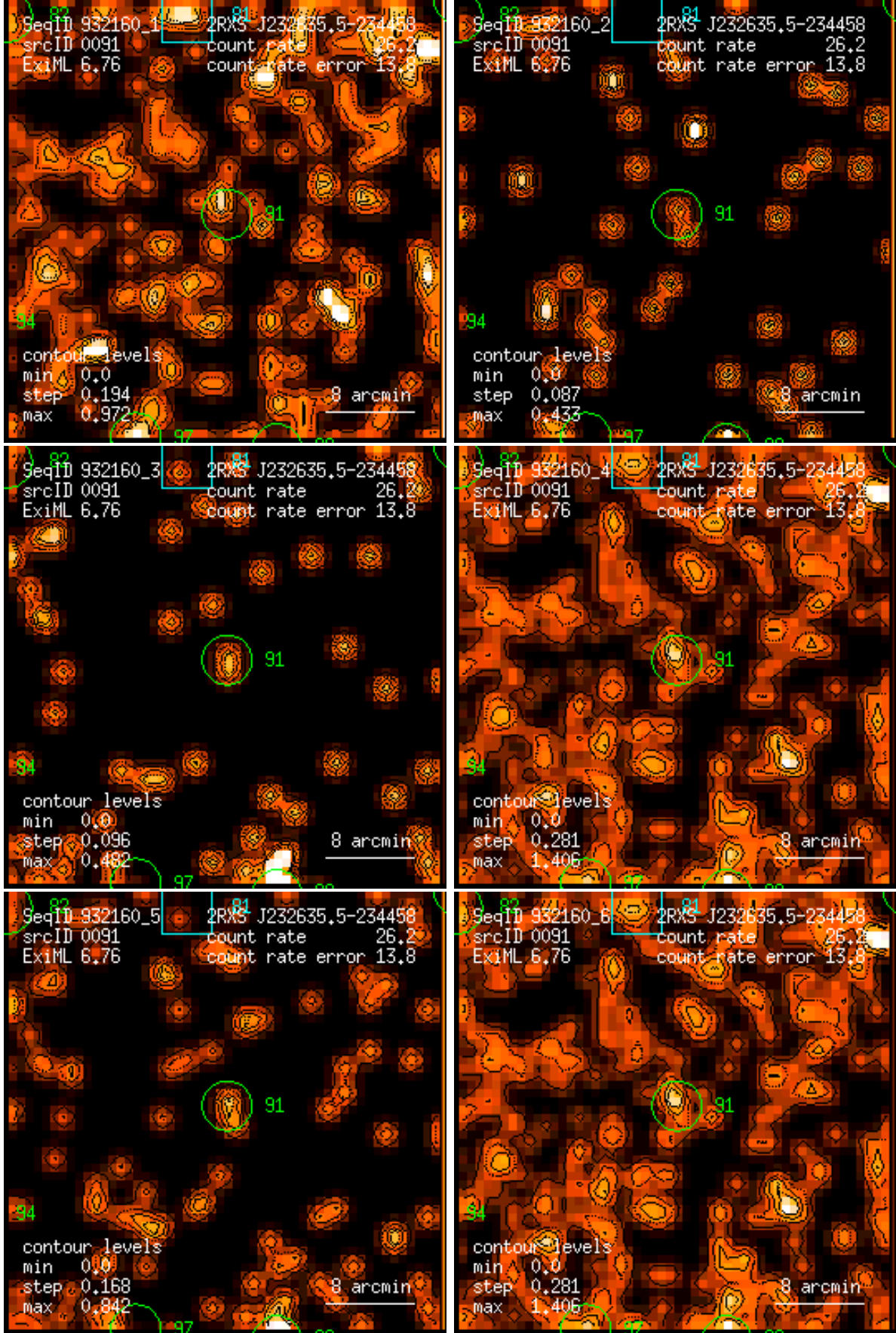
Figure 91: RASS 932160: detection 0091: band rate images, Gaussian filter: (1) PSPC channels 11 – 41, (2) 52 – 90, (3) 91 – 201, (4) 11 – 235, (5) 52 – 201, (6) 11 – 201. Broad band rates in counts/ks. Band rate contour levels in counts/ks/arcmin 2 .
