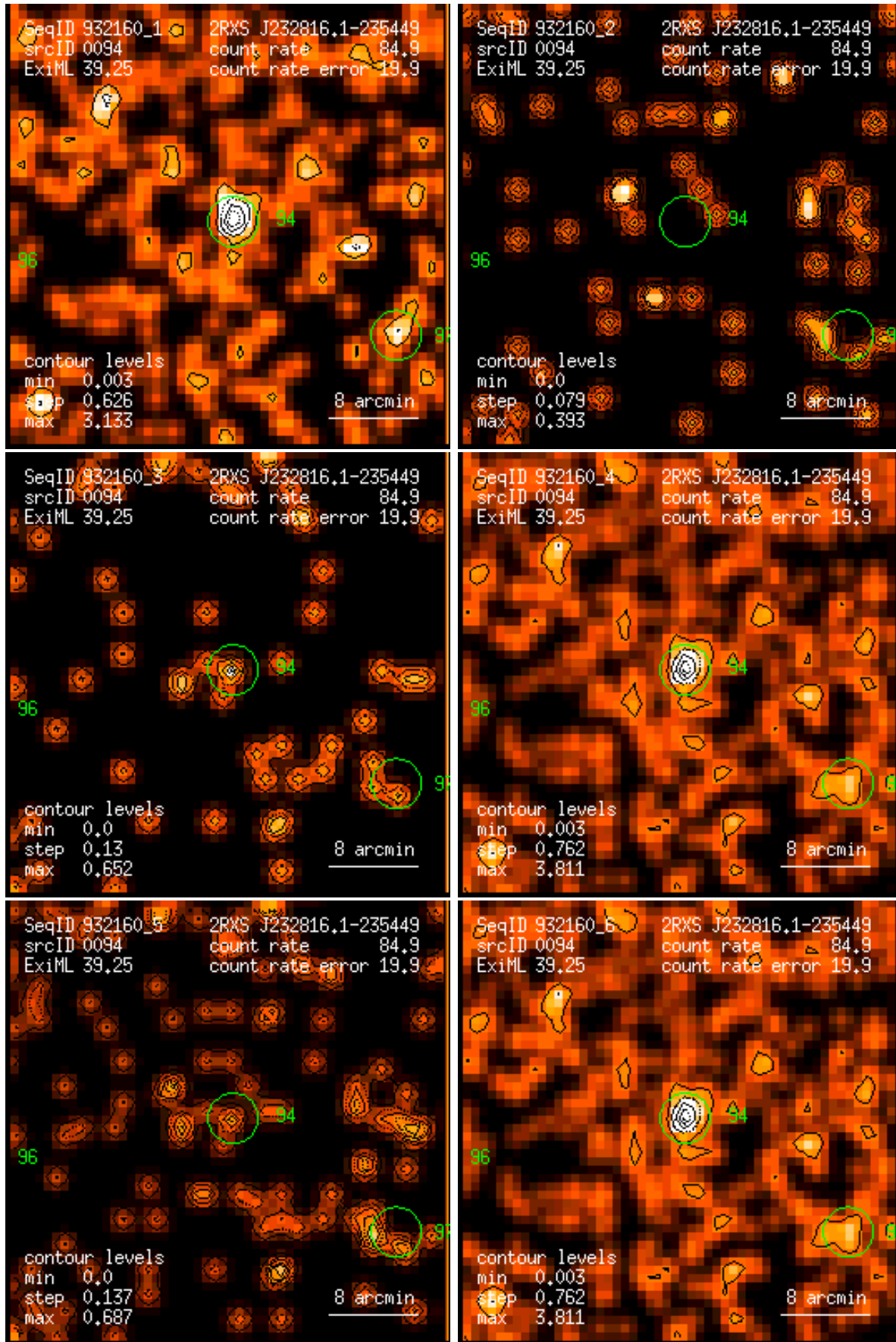
Figure 94: RASS 932160: detection 0094: band rate images, Gaussian filter: (1) PSPC channels 11 – 41, (2) 52 – 90, (3) 91 – 201, (4) 11 – 235, (5) 52 – 201, (6) 11 – 201. Broad band rates in counts/ks. Band rate contour levels in counts/ks/arcmin 2 .
