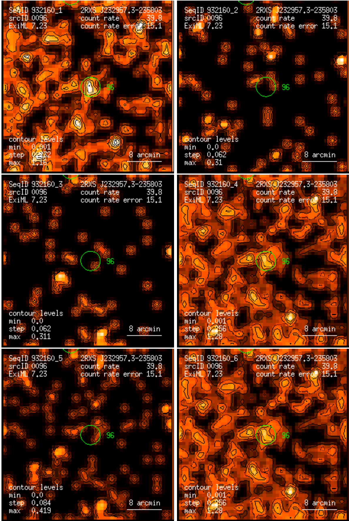
Figure 96: RASS 932160: detection 0096: band rate images, Gaussian filter: (1) PSPC channels 11 – 41, (2) 52 – 90, (3) 91 – 201, (4) 11 – 235, (5) 52 – 201, (6) 11 – 201. Broad band rates in counts/ks. Band rate contour levels in counts/ks/arcmin 2 .
