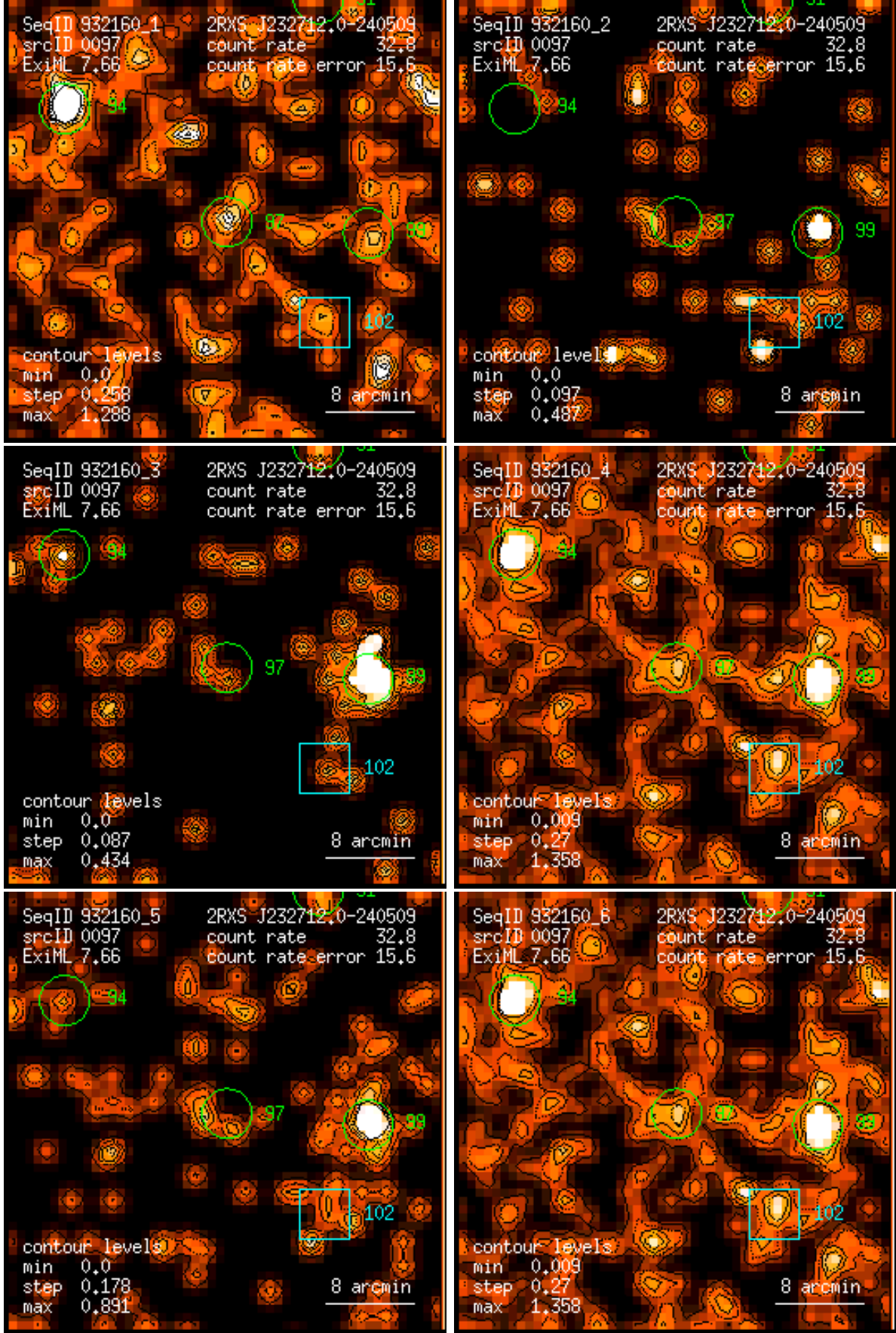
Figure 97: RASS 932160: detection 0097: band rate images, Gaussian filter: (1) PSPC channels 11 – 41, (2) 52 – 90, (3) 91 – 201, (4) 11 – 235, (5) 52 – 201, (6) 11 – 201. Broad band rates in counts/ks. Band rate contour levels in counts/ks/arcmin 2 .
