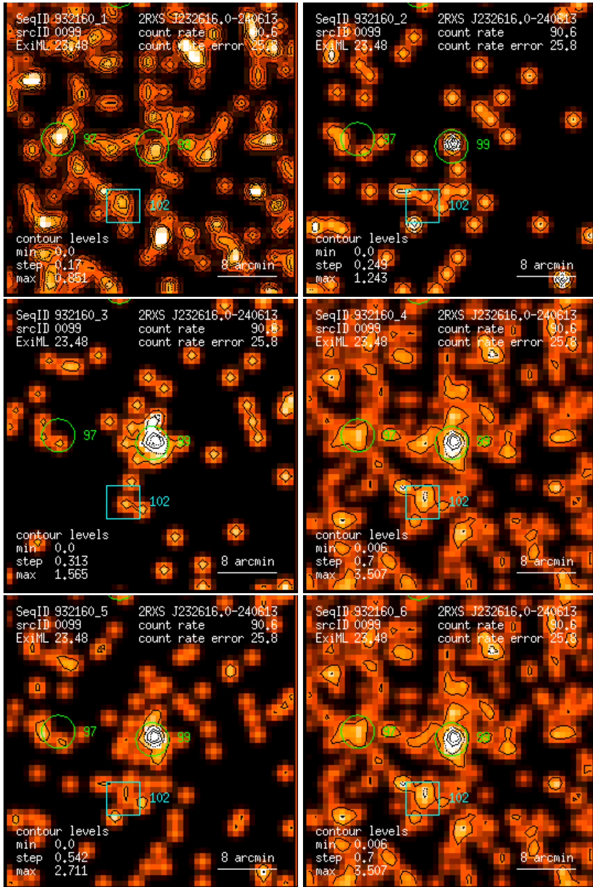
Figure 99: RASS 932160: detection 0099: band rate images, Gaussian filter: (1) PSPC channels 11 – 41, (2) 52 – 90, (3) 91 – 201, (4) 11 – 235, (5) 52 – 201, (6) 11 – 201. Broad band rates in counts/ks. Band rate contour levels in counts/ks/arcmin 2 .
