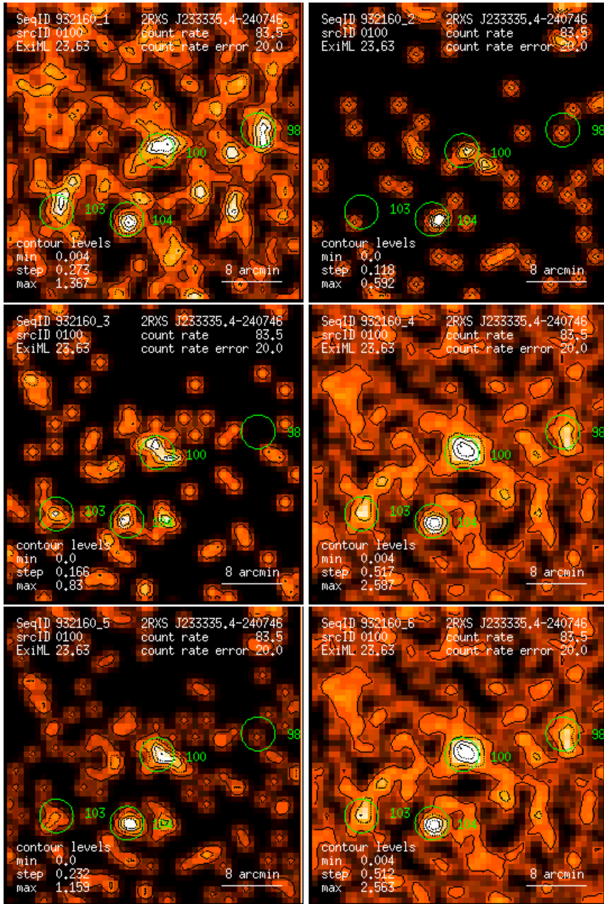
Figure 100: RASS 932160: detection 0100: band rate images, Gaussian filter: (1) PSPC channels 11 – 41, (2) 52 – 90, (3) 91 – 201, (4) 11 – 235, (5) 52 – 201, (6) 11 – 201. Broad band rates in counts/ks. Band rate contour levels in counts/ks/arcmin 2 .
