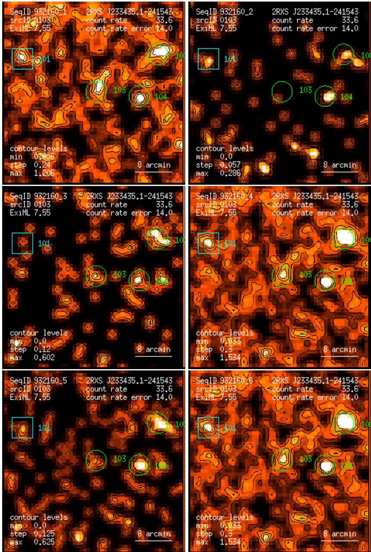
Figure 103: RASS 932160: detection 0103: band rate images, Gaussian filter: (1) PSPC channels 11 – 41, (2) 52 – 90, (3) 91 – 201, (4) 11 – 235, (5) 52 – 201, (6) 11 – 201. Broad band rates in counts/ks. Band rate contour levels in counts/ks/arcmin 2 .
