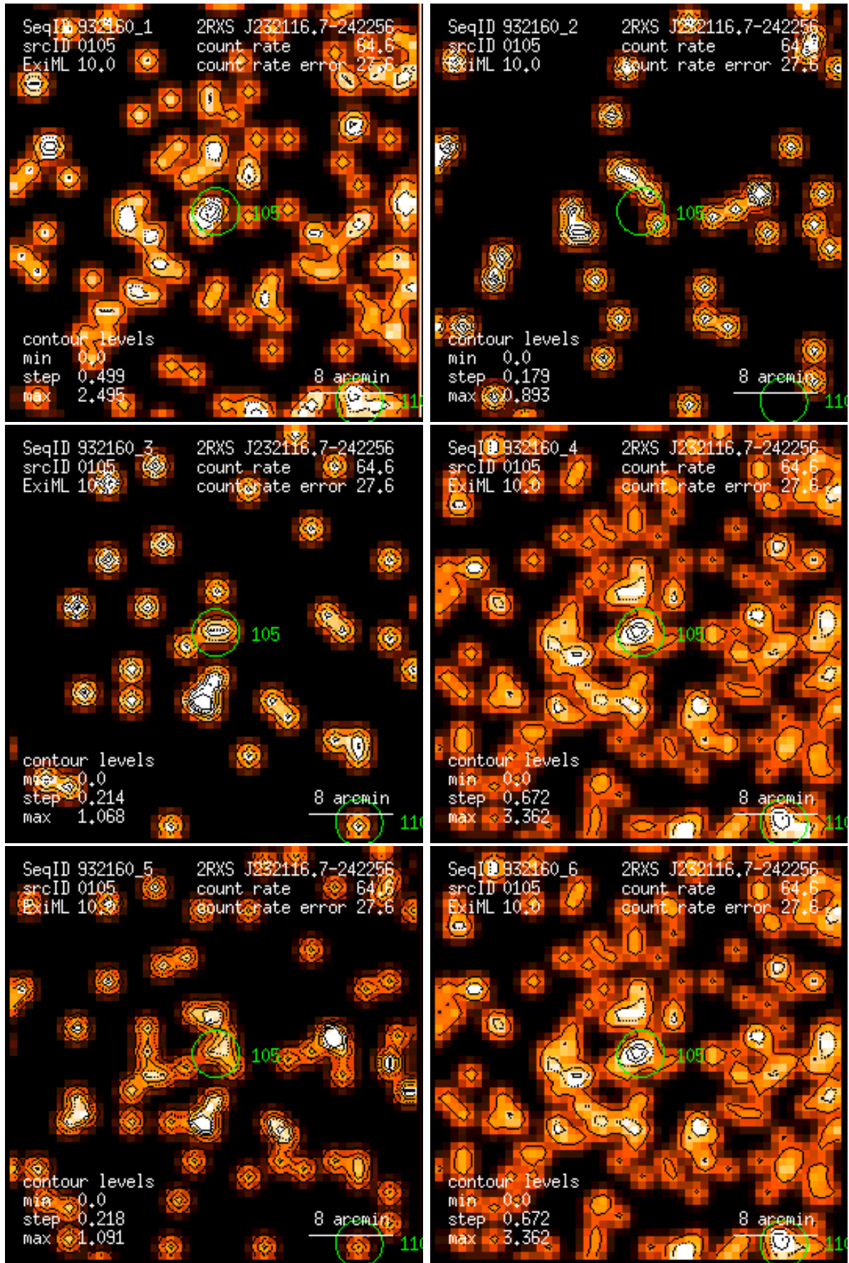
Figure 105: RASS 932160: detection 0105: band rate images, Gaussian filter: (1) PSPC channels 11 – 41, (2) 52 – 90, (3) 91 – 201, (4) 11 – 235, (5) 52 – 201, (6) 11 – 201. Broad band rates in counts/ks. Band rate contour levels in counts/ks/arcmin 2 .
