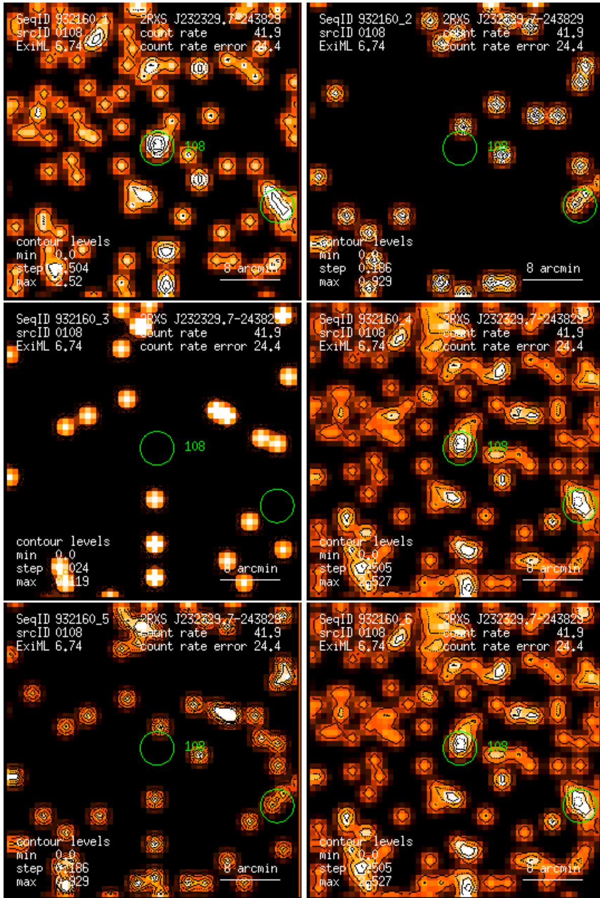
Figure 108: RASS 932160: detection 0108: band rate images, Gaussian filter: (1) PSPC channels 11 – 41, (2) 52 – 90, (3) 91 – 201, (4) 11 – 235, (5) 52 – 201, (6) 11 – 201. Broad band rates in counts/ks. Band rate contour levels in counts/ks/arcmin 2 .
