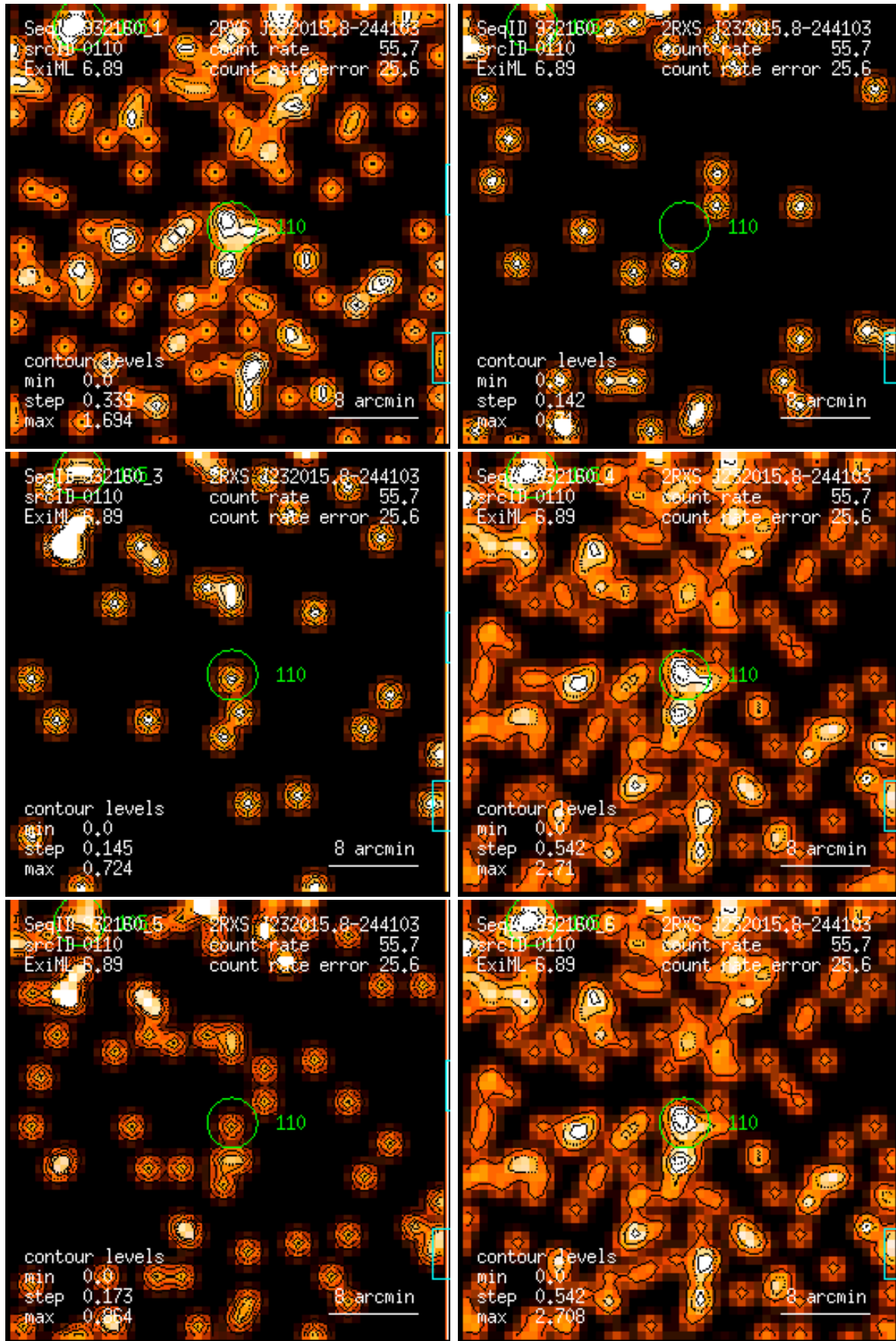
Figure 110: RASS 932160: detection 0110: band rate images, Gaussian filter: (1) PSPC channels 11 – 41, (2) 52 – 90, (3) 91 – 201, (4) 11 – 235, (5) 52 – 201, (6) 11 – 201. Broad band rates in counts/ks. Band rate contour levels in counts/ks/arcmin 2 .
