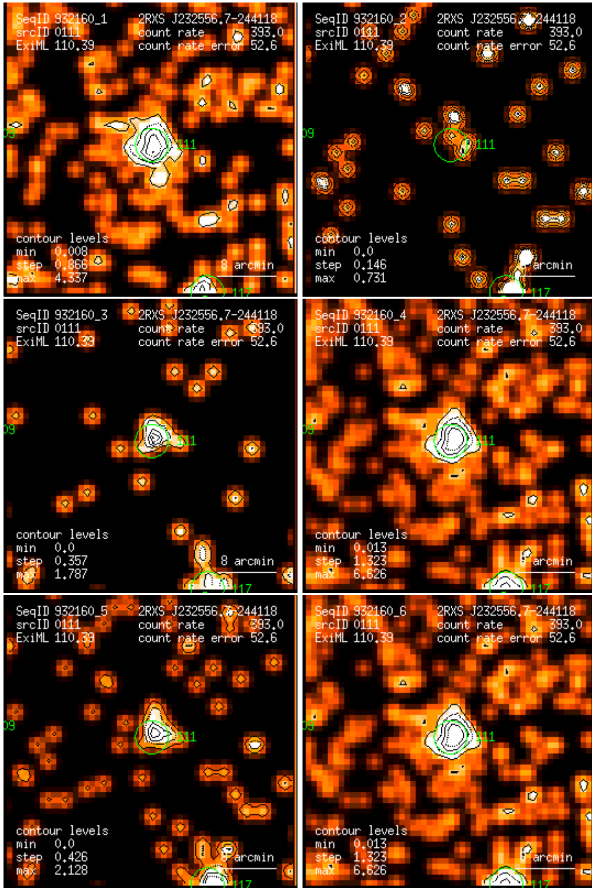
Figure 111: RASS 932160: detection 0111: band rate images, Gaussian filter: (1) PSPC channels 11 – 41, (2) 52 – 90, (3) 91 – 201, (4) 11 – 235, (5) 52 – 201, (6) 11 – 201. Broad band rates in counts/ks. Band rate contour levels in counts/ks/arcmin 2 .
