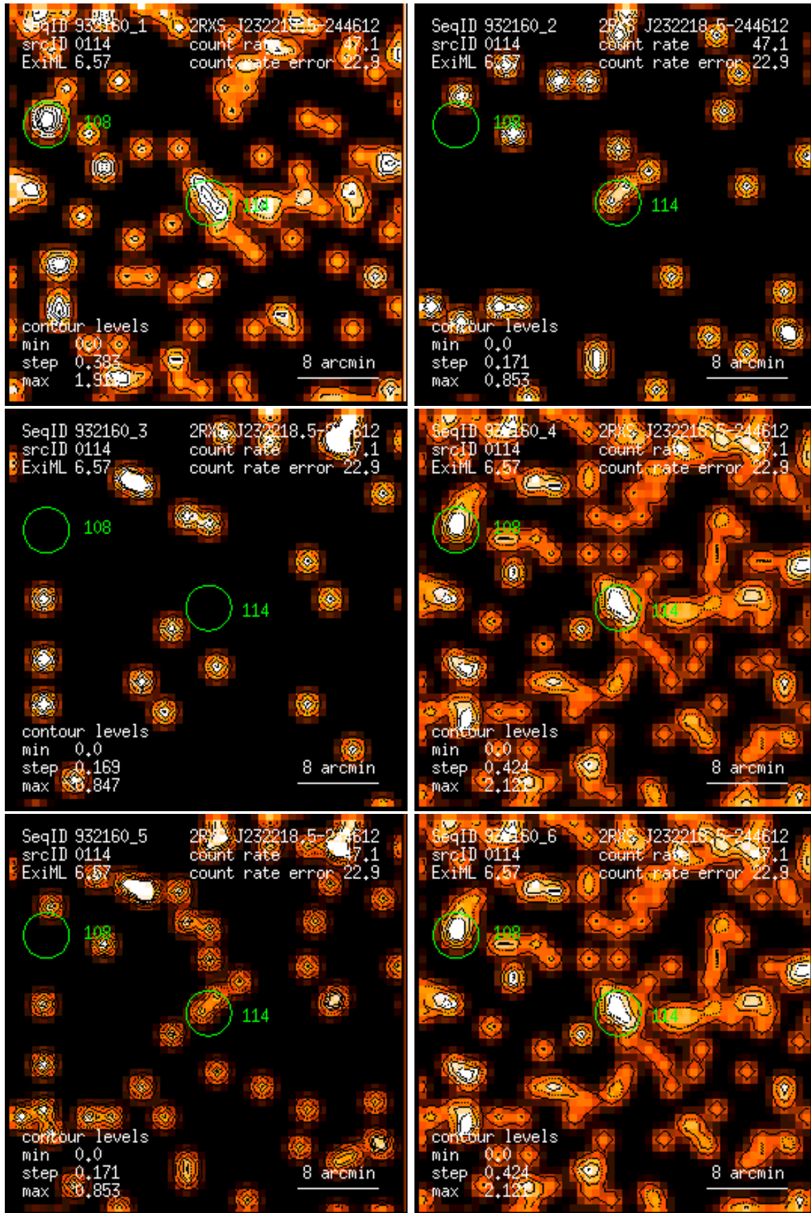
Figure 114: RASS 932160: detection 0114: band rate images, Gaussian filter: (1) PSPC channels 11 – 41, (2) 52 – 90, (3) 91 – 201, (4) 11 – 235, (5) 52 – 201, (6) 11 – 201. Broad band rates in counts/ks. Band rate contour levels in counts/ks/arcmin 2 .
