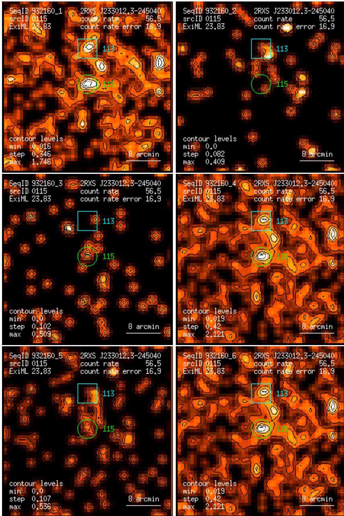
Figure 115: RASS 932160: detection 0115: band rate images, Gaussian filter: (1) PSPC channels 11 – 41, (2) 52 – 90, (3) 91 – 201, (4) 11 – 235, (5) 52 – 201, (6) 11 – 201. Broad band rates in counts/ks. Band rate contour levels in counts/ks/arcmin 2 .
