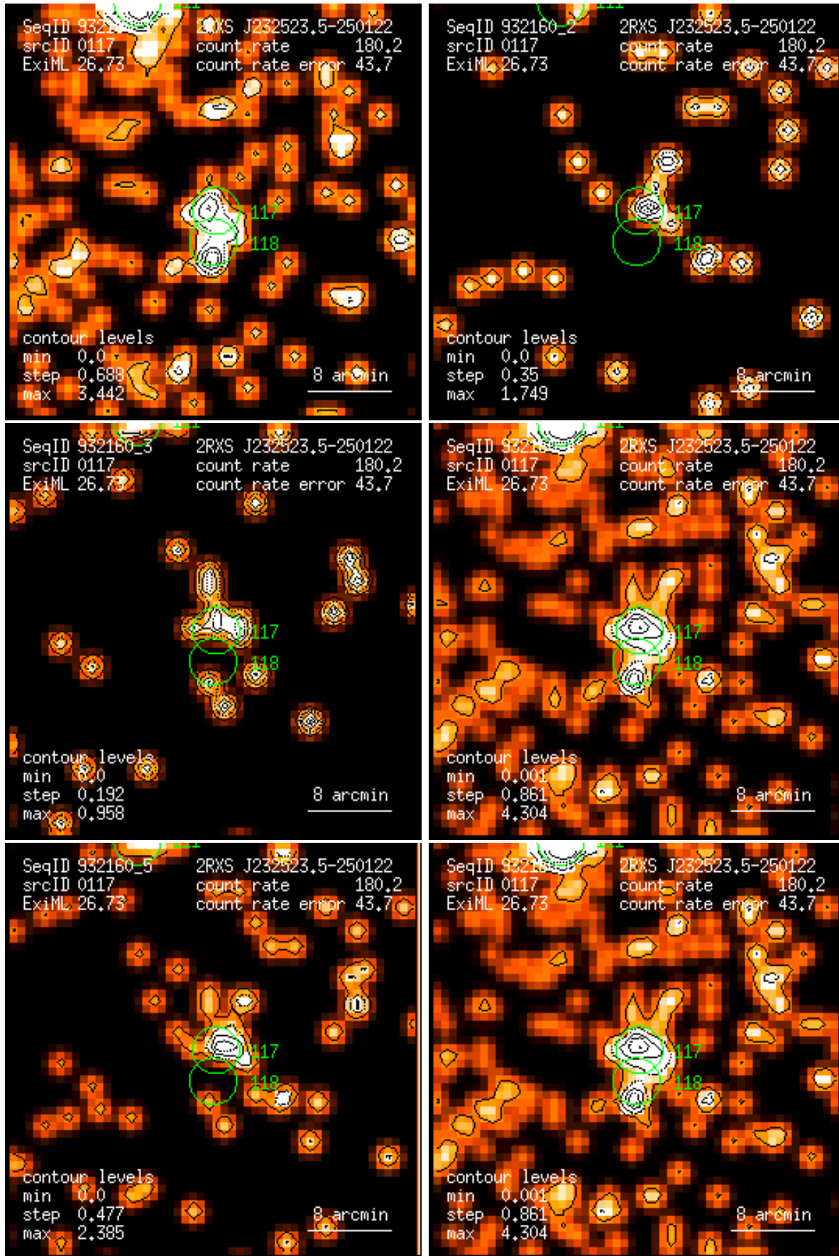
Figure 117: RASS 932160: detection 0117: band rate images, Gaussian filter: (1) PSPC channels 11 – 41, (2) 52 – 90, (3) 91 – 201, (4) 11 – 235, (5) 52 – 201, (6) 11 – 201. Broad band rates in counts/ks. Band rate contour levels in counts/ks/arcmin 2 .
