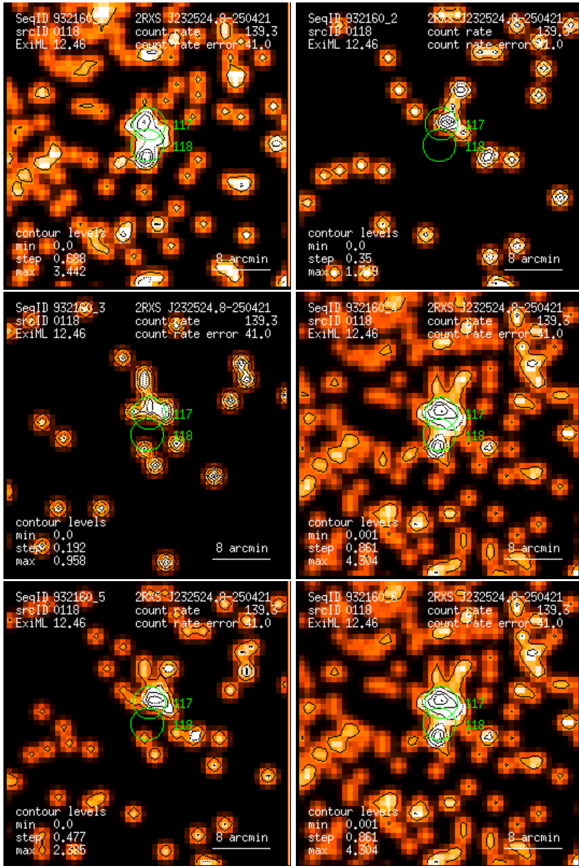
Figure 118: RASS 932160: detection 0118: band rate images, Gaussian filter: (1) PSPC channels 11 – 41, (2) 52 – 90, (3) 91 – 201, (4) 11 – 235, (5) 52 – 201, (6) 11 – 201. Broad band rates in counts/ks. Band rate contour levels in counts/ks/arcmin 2 .
