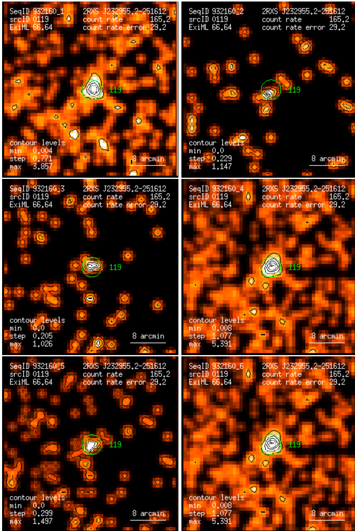
Figure 119: RASS 932160: detection 0119: band rate images, Gaussian filter: (1) PSPC channels 11 – 41, (2) 52 – 90, (3) 91 – 201, (4) 11 – 235, (5) 52 – 201, (6) 11 – 201. Broad band rates in counts/ks. Band rate contour levels in counts/ks/arcmin 2 .
