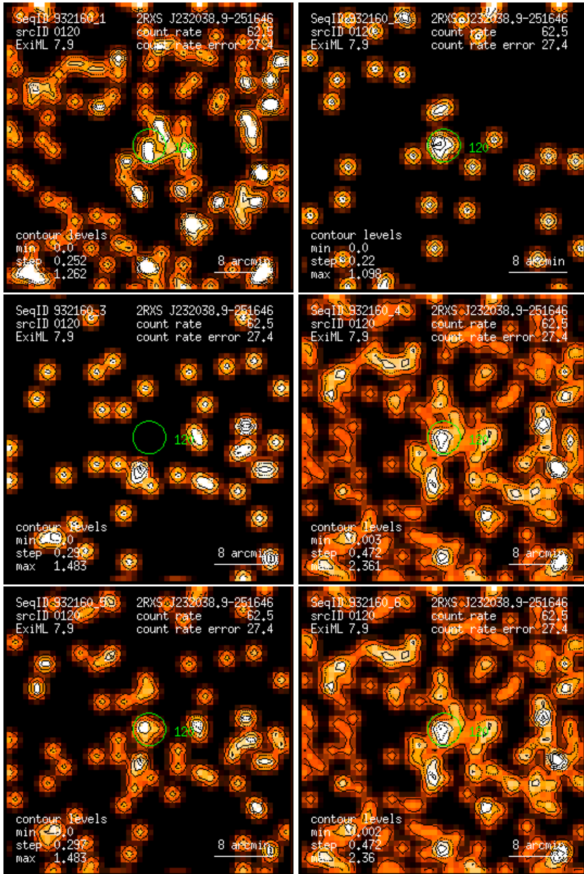
Figure 120: RASS 932160: detection 0120: band rate images, Gaussian filter: (1) PSPC channels 11 – 41, (2) 52 – 90, (3) 91 – 201, (4) 11 – 235, (5) 52 – 201, (6) 11 – 201. Broad band rates in counts/ks. Band rate contour levels in counts/ks/arcmin 2 .
