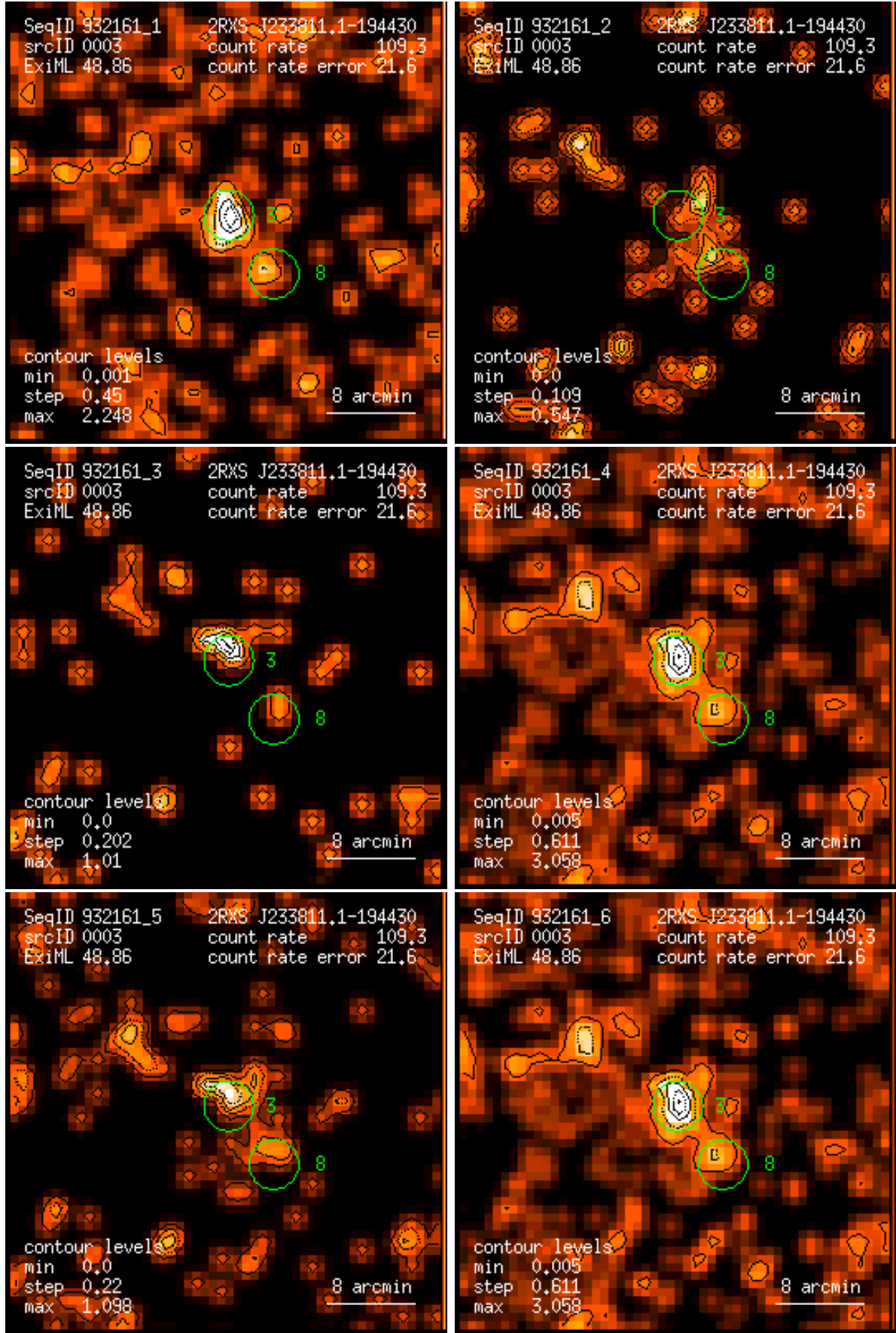
Figure 3: RASS 932161: detection 0003: band rate images, Gaussian filter: (1) PSPC channels 11 – 41, (2) 52 – 90, (3) 91 – 201, (4) 11 – 235, (5) 52 – 201, (6) 11 – 201. Broad band rates in counts/ks. Band rate contour levels in counts/ks/arcmin 2 .
