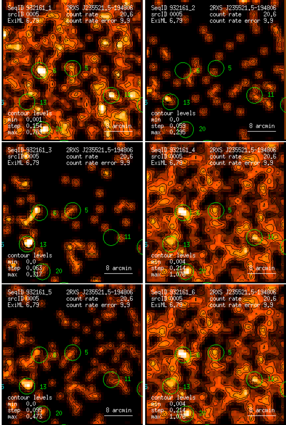
Figure 5: RASS 932161: detection 0005: band rate images, Gaussian filter: (1) PSPC channels 11 – 41, (2) 52 – 90, (3) 91 – 201, (4) 11 – 235, (5) 52 – 201, (6) 11 – 201. Broad band rates in counts/ks. Band rate contour levels in counts/ks/arcmin 2 .
