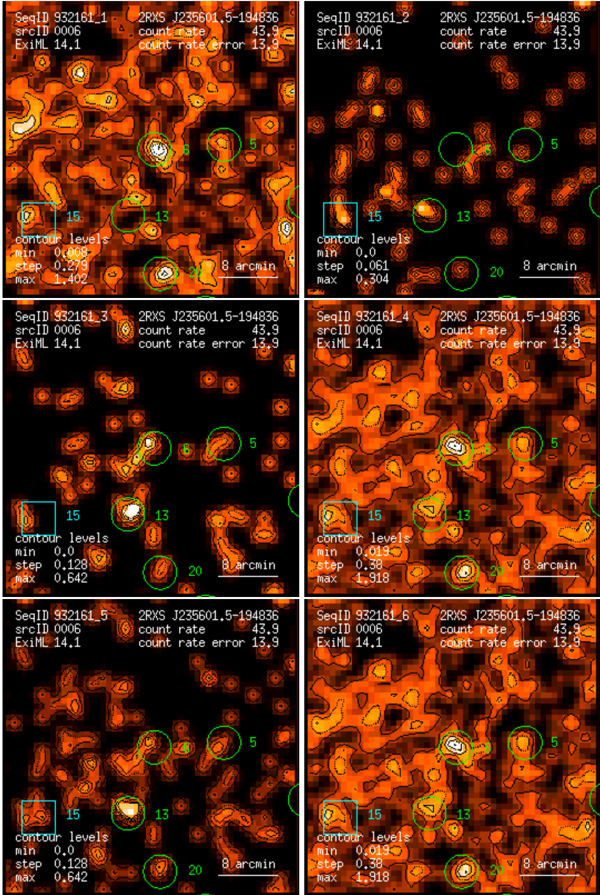
Figure 6: RASS 932161: detection 0006: band rate images, Gaussian filter: (1) PSPC channels 11 – 41, (2) 52 – 90, (3) 91 – 201, (4) 11 – 235, (5) 52 – 201, (6) 11 – 201. Broad band rates in counts/ks. Band rate contour levels in counts/ks/arcmin 2 .
