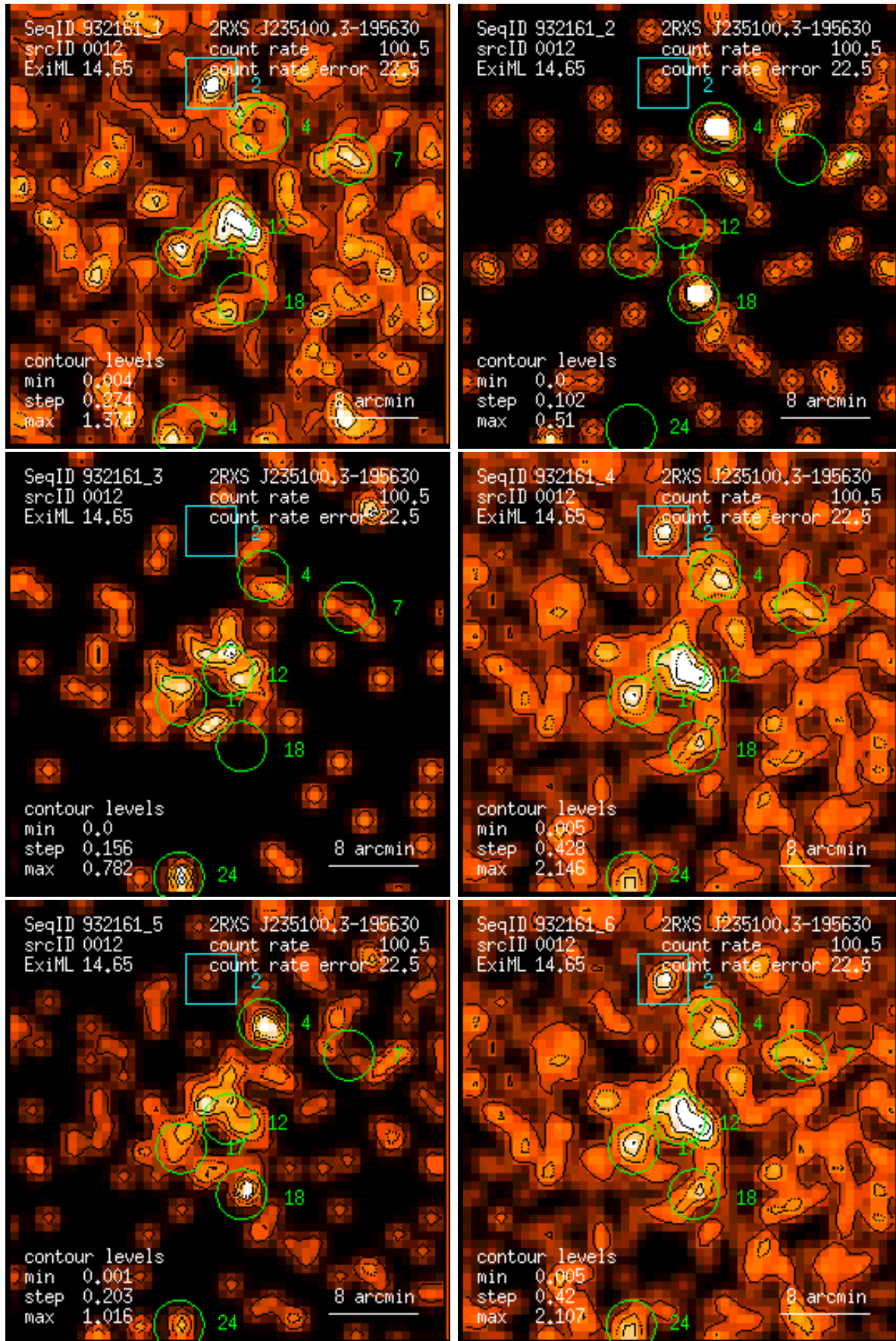
Figure 12: RASS 932161: detection 0012: band rate images, Gaussian filter: (1) PSPC channels 11 – 41, (2) 52 – 90, (3) 91 – 201, (4) 11 – 235, (5) 52 – 201, (6) 11 – 201. Broad band rates in counts/ks. Band rate contour levels in counts/ks/arcmin 2 .
