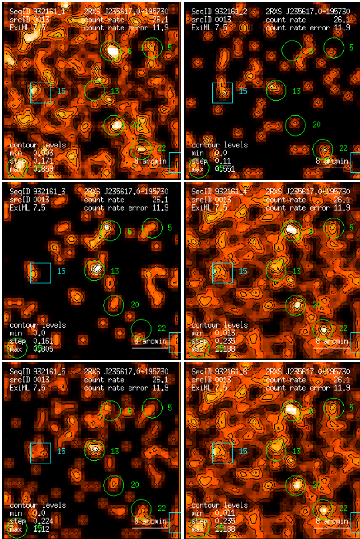
Figure 13: RASS 932161: detection 0013: band rate images, Gaussian filter: (1) PSPC channels 11 – 41, (2) 52 – 90, (3) 91 – 201, (4) 11 – 235, (5) 52 – 201, (6) 11 – 201. Broad band rates in counts/ks. Band rate contour levels in counts/ks/arcmin 2 .
