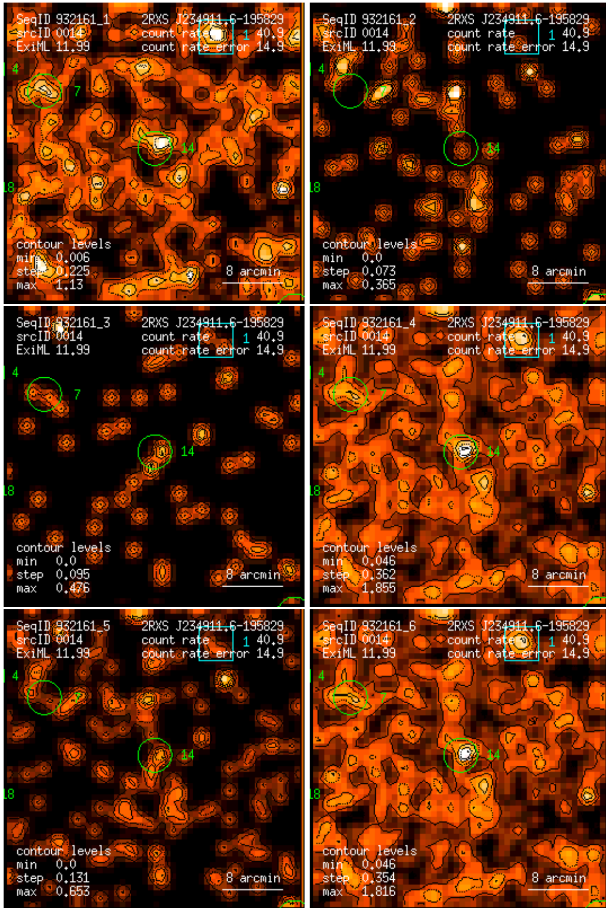
Figure 14: RASS 932161: detection 0014: band rate images, Gaussian filter: (1) PSPC channels 11 – 41, (2) 52 – 90, (3) 91 – 201, (4) 11 – 235, (5) 52 – 201, (6) 11 – 201. Broad band rates in counts/ks. Band rate contour levels in counts/ks/arcmin 2 .
