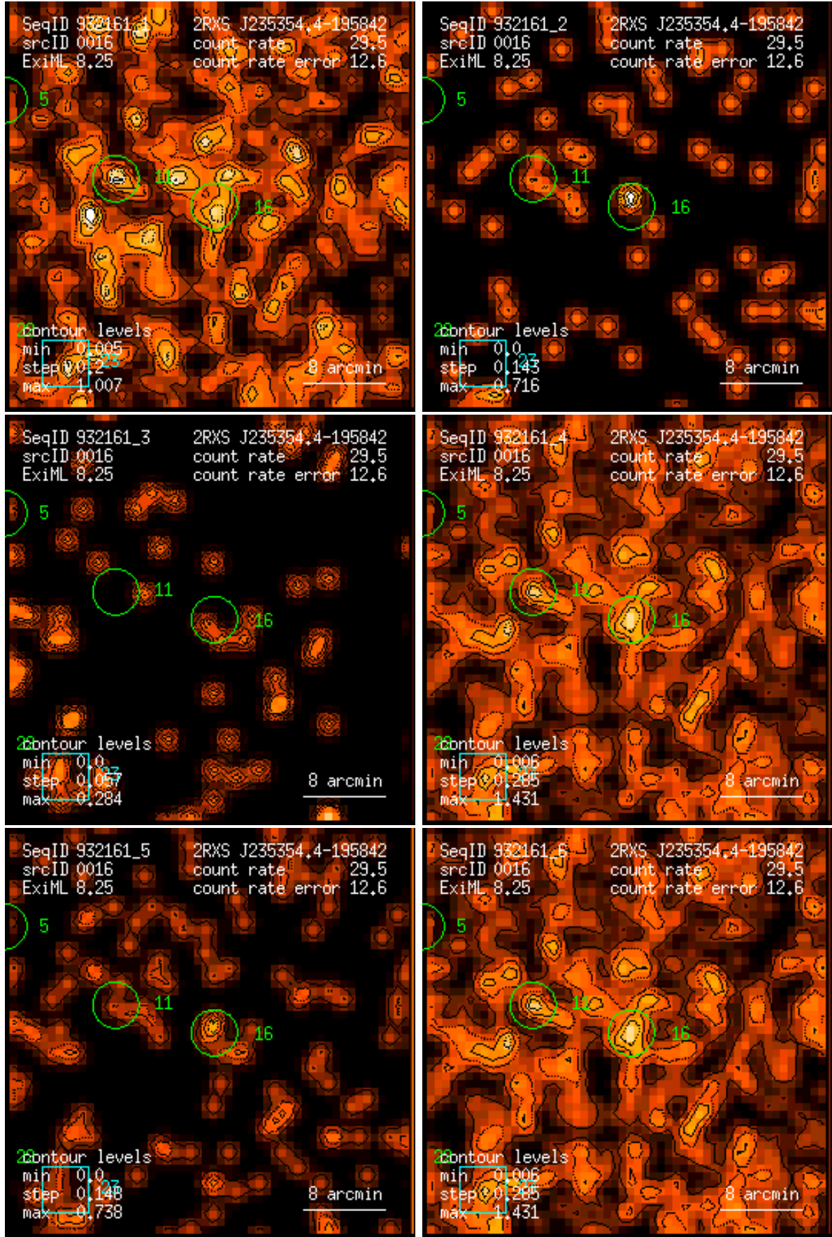
Figure 16: RASS 932161: detection 0016: band rate images, Gaussian filter: (1) PSPC channels 11 – 41, (2) 52 – 90, (3) 91 – 201, (4) 11 – 235, (5) 52 – 201, (6) 11 – 201. Broad band rates in counts/ks. Band rate contour levels in counts/ks/arcmin 2 .
