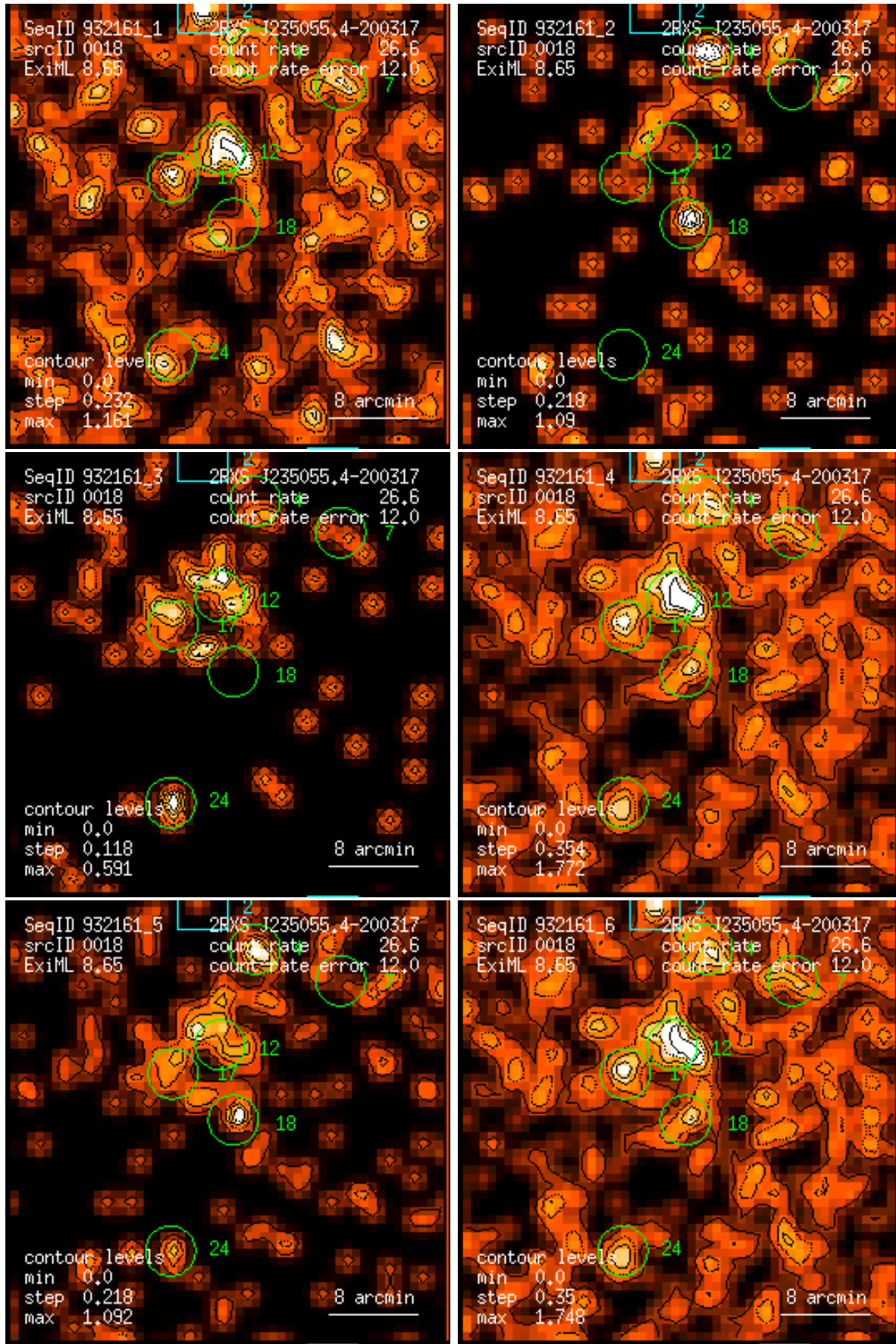
Figure 18: RASS 932161: detection 0018: band rate images, Gaussian filter: (1) PSPC channels 11 – 41, (2) 52 – 90, (3) 91 – 201, (4) 11 – 235, (5) 52 – 201, (6) 11 – 201. Broad band rates in counts/ks. Band rate contour levels in counts/ks/arcmin 2 .
