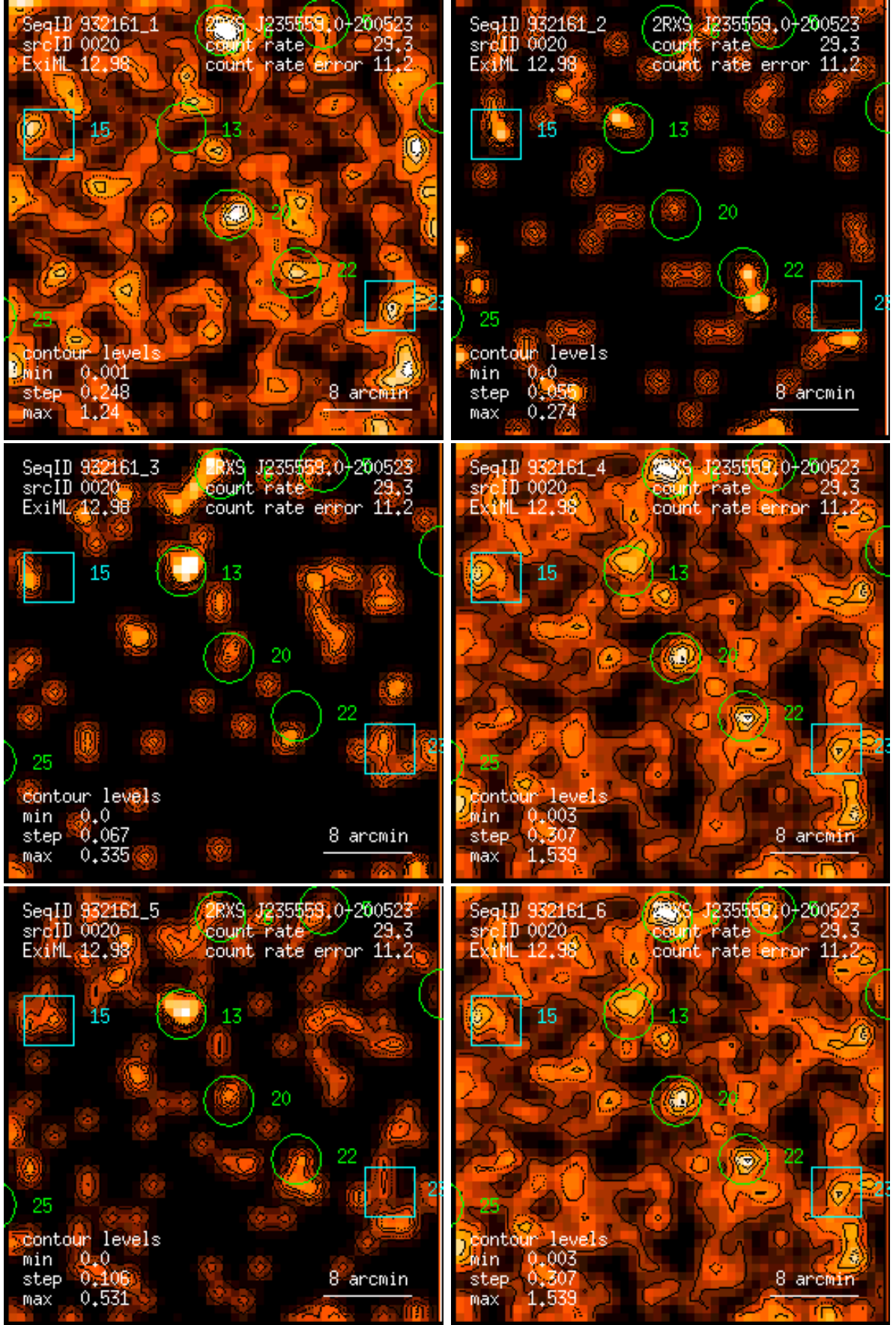
Figure 20: RASS 932161: detection 0020: band rate images, Gaussian filter: (1) PSPC channels 11 – 41, (2) 52 – 90, (3) 91 – 201, (4) 11 – 235, (5) 52 – 201, (6) 11 – 201. Broad band rates in counts/ks. Band rate contour levels in counts/ks/arcmin 2 .
