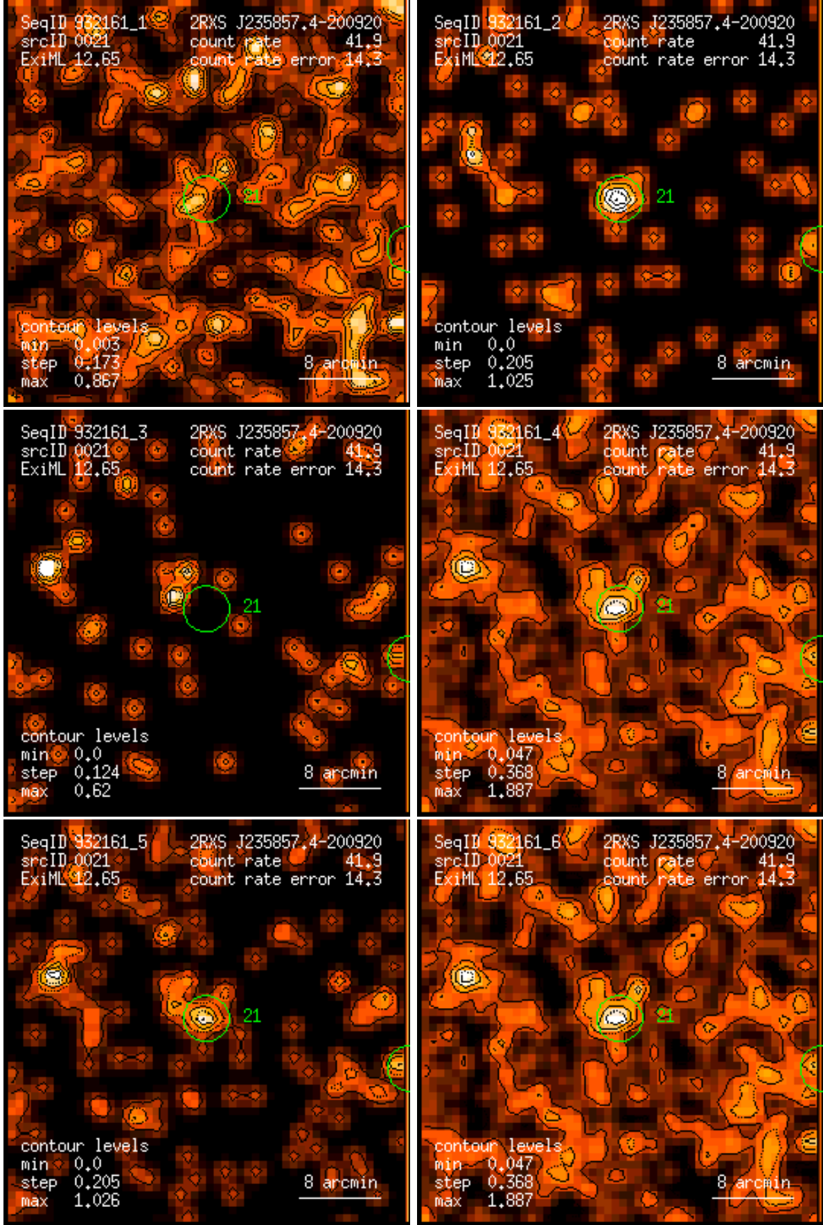
Figure 21: RASS 932161: detection 0021: band rate images, Gaussian filter: (1) PSPC channels 11 – 41, (2) 52 – 90, (3) 91 – 201, (4) 11 – 235, (5) 52 – 201, (6) 11 – 201. Broad band rates in counts/ks. Band rate contour levels in counts/ks/arcmin 2 .
