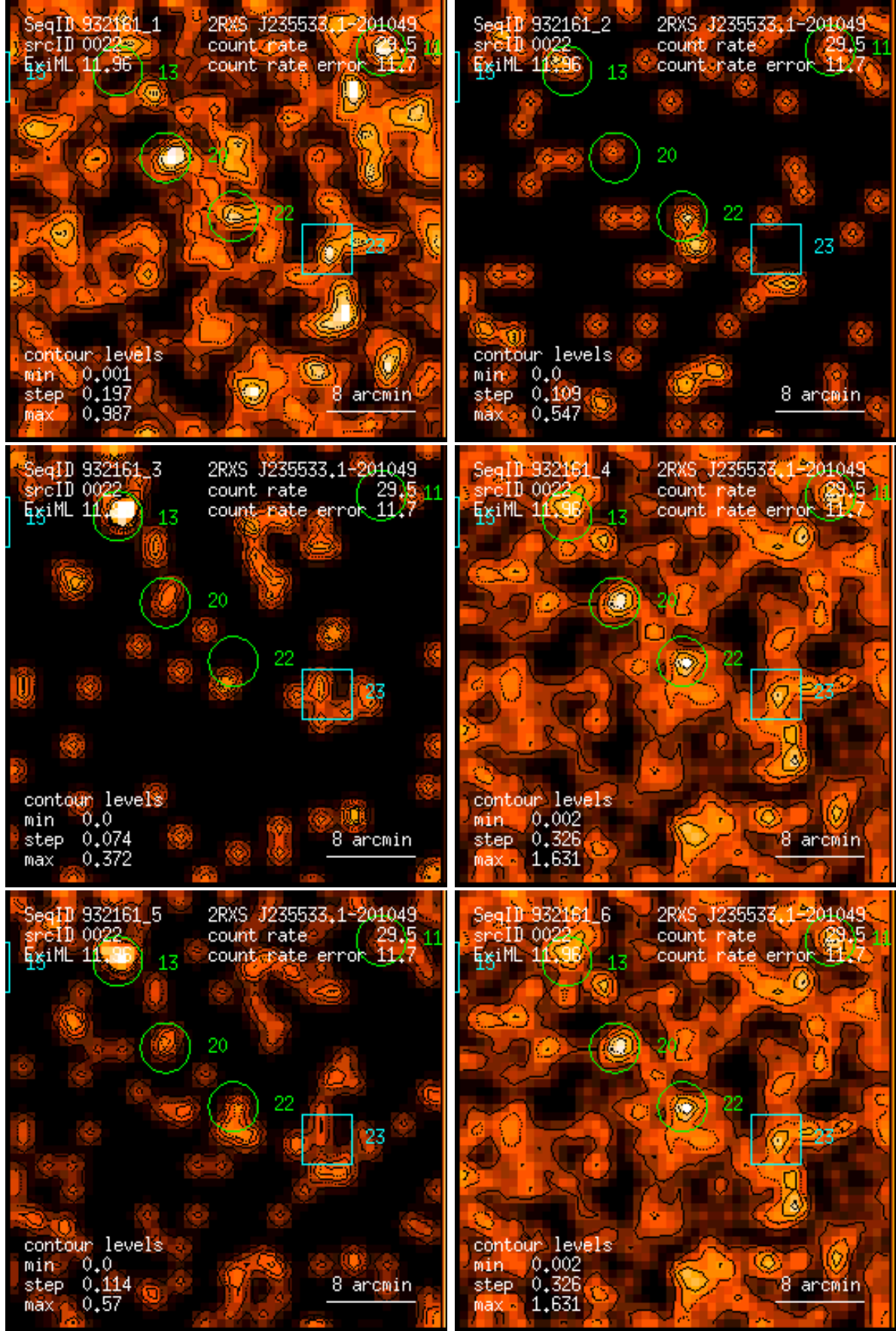
Figure 22: RASS 932161: detection 0022: band rate images, Gaussian filter: (1) PSPC channels 11 – 41, (2) 52 – 90, (3) 91 – 201, (4) 11 – 235, (5) 52 – 201, (6) 11 – 201. Broad band rates in counts/ks. Band rate contour levels in counts/ks/arcmin 2 .
