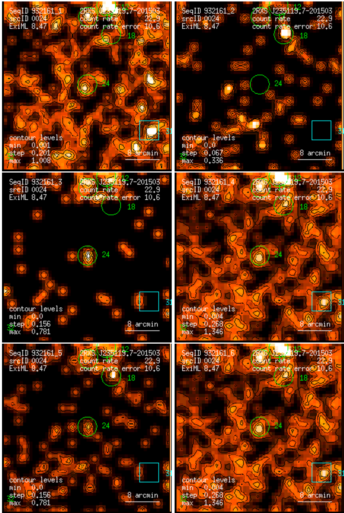
Figure 24: RASS 932161: detection 0024: band rate images, Gaussian filter: (1) PSPC channels 11 – 41, (2) 52 – 90, (3) 91 – 201, (4) 11 – 235, (5) 52 – 201, (6) 11 – 201. Broad band rates in counts/ks. Band rate contour levels in counts/ks/arcmin 2 .
