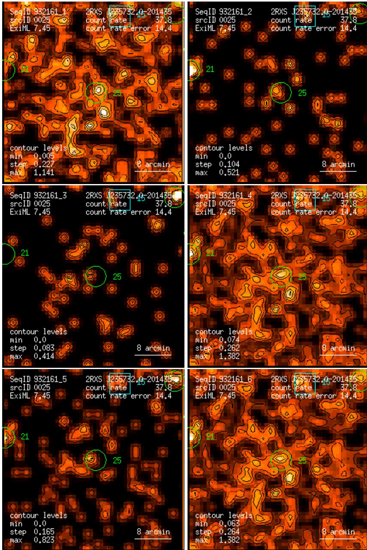
Figure 25: RASS 932161: detection 0025: band rate images, Gaussian filter: (1) PSPC channels 11 – 41, (2) 52 – 90, (3) 91 – 201, (4) 11 – 235, (5) 52 – 201, (6) 11 – 201. Broad band rates in counts/ks. Band rate contour levels in counts/ks/arcmin 2 .
