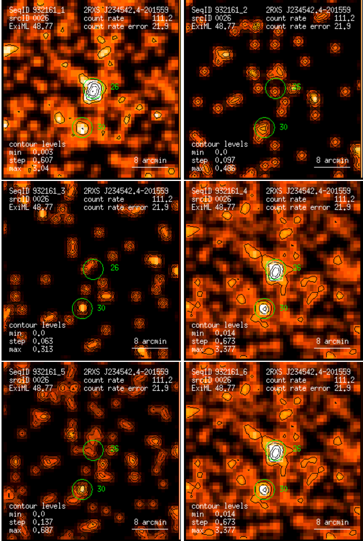
Figure 26: RASS 932161: detection 0026: band rate images, Gaussian filter: (1) PSPC channels 11 – 41, (2) 52 – 90, (3) 91 – 201, (4) 11 – 235, (5) 52 – 201, (6) 11 – 201. Broad band rates in counts/ks. Band rate contour levels in counts/ks/arcmin 2 .
