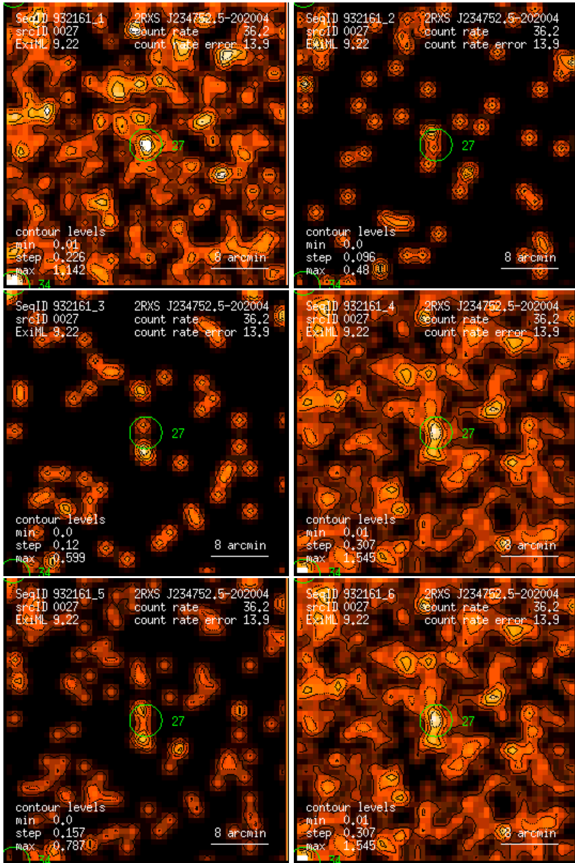
Figure 27: RASS 932161: detection 0027: band rate images, Gaussian filter: (1) PSPC channels 11 – 41, (2) 52 – 90, (3) 91 – 201, (4) 11 – 235, (5) 52 – 201, (6) 11 – 201. Broad band rates in counts/ks. Band rate contour levels in counts/ks/arcmin 2 .
