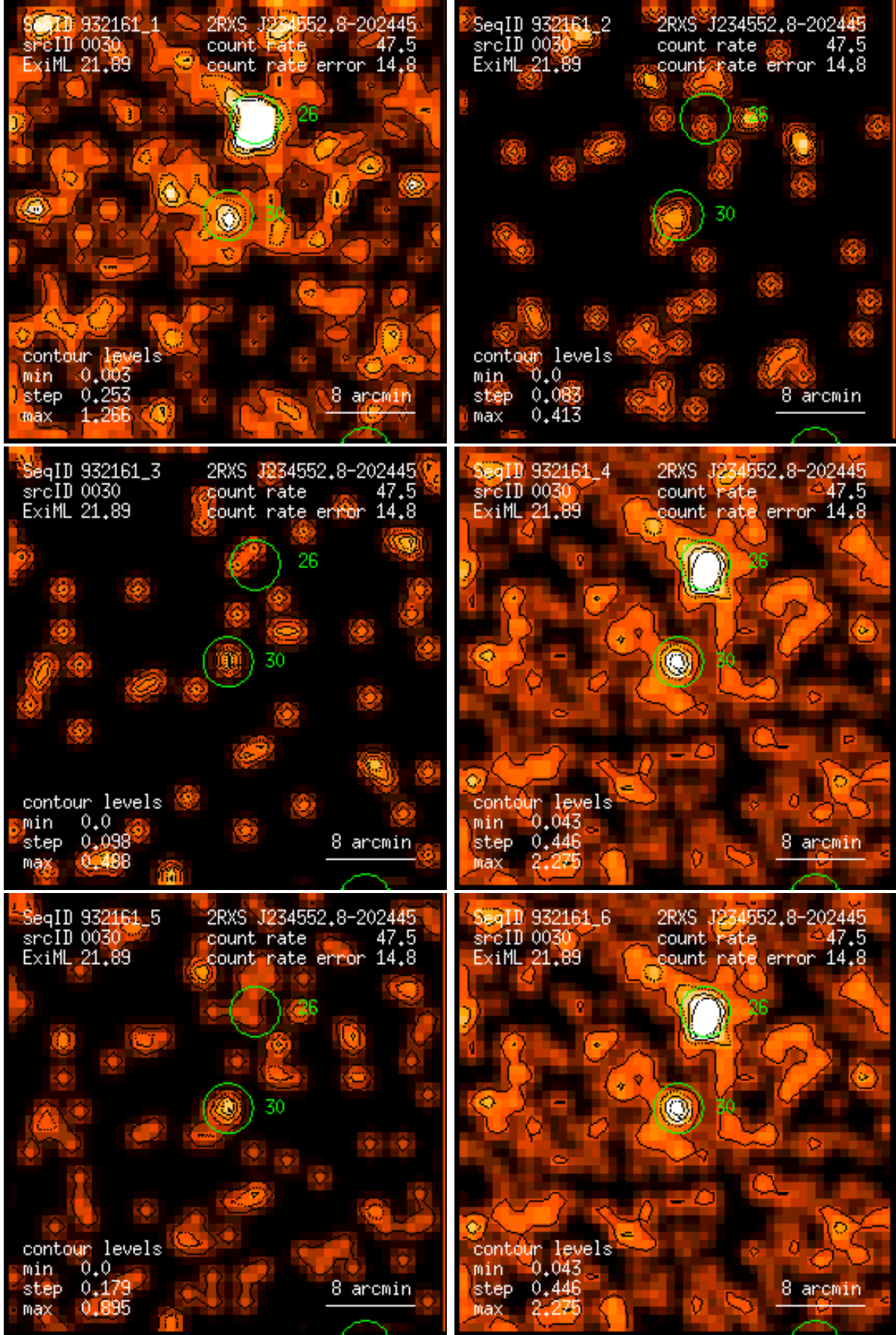
Figure 30: RASS 932161: detection 0030: band rate images, Gaussian filter: (1) PSPC channels 11 – 41, (2) 52 – 90, (3) 91 – 201, (4) 11 – 235, (5) 52 – 201, (6) 11 – 201. Broad band rates in counts/ks. Band rate contour levels in counts/ks/arcmin 2 .
