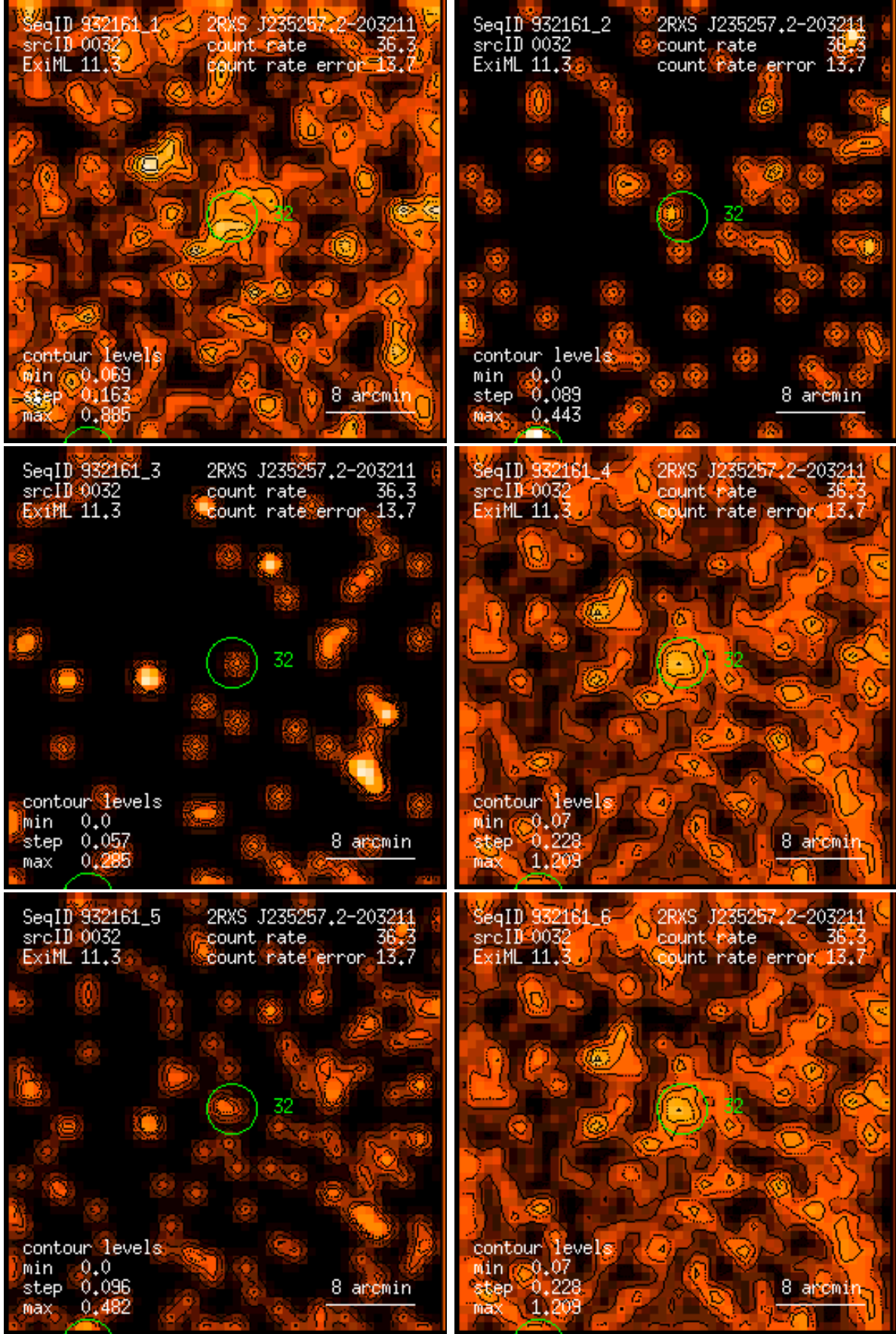
Figure 32: RASS 932161: detection 0032: band rate images, Gaussian filter: (1) PSPC channels 11 – 41, (2) 52 – 90, (3) 91 – 201, (4) 11 – 235, (5) 52 – 201, (6) 11 – 201. Broad band rates in counts/ks. Band rate contour levels in counts/ks/arcmin 2 .
