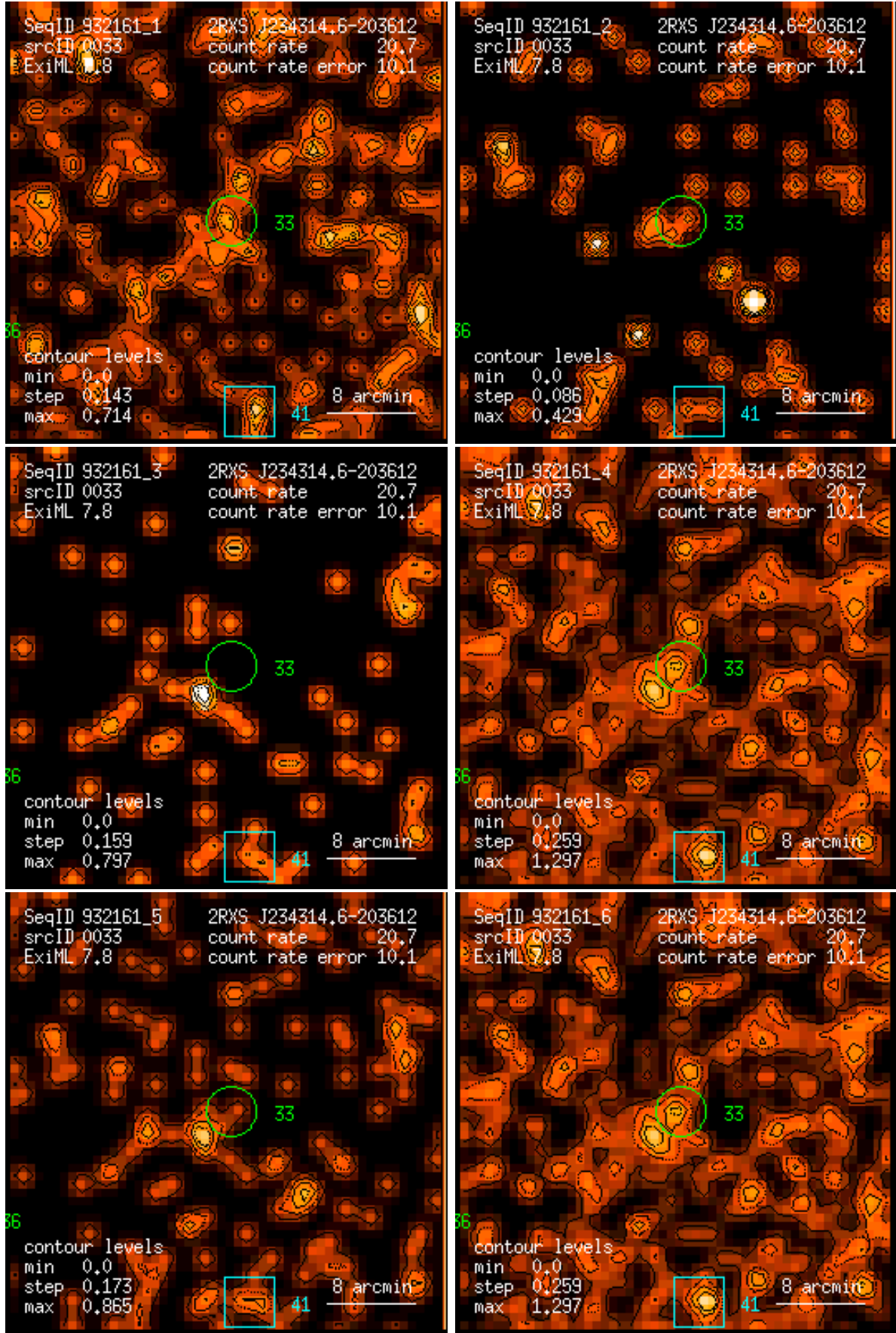
Figure 33: RASS 932161: detection 0033: band rate images, Gaussian filter: (1) PSPC channels 11 – 41, (2) 52 – 90, (3) 91 – 201, (4) 11 – 235, (5) 52 – 201, (6) 11 – 201. Broad band rates in counts/ks. Band rate contour levels in counts/ks/arcmin 2 .
