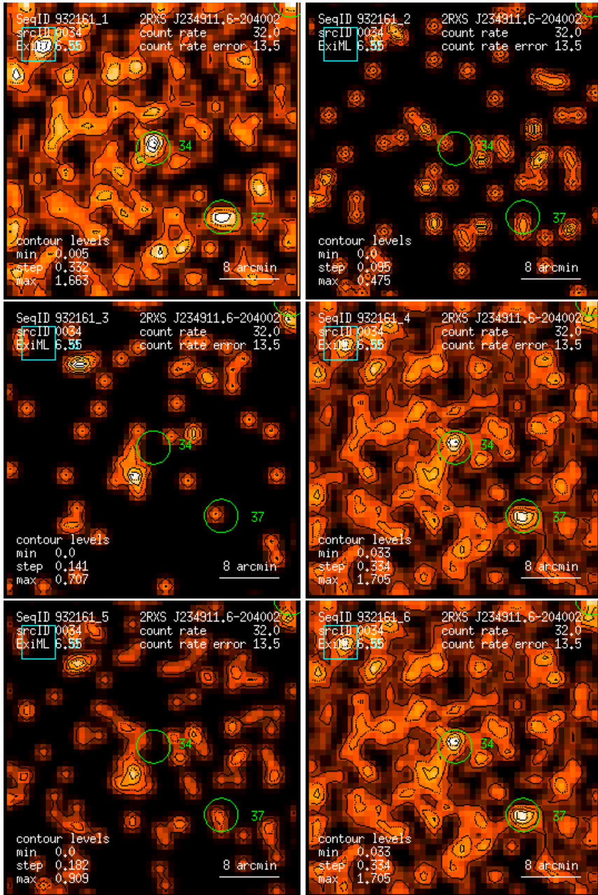
Figure 34: RASS 932161: detection 0034: band rate images, Gaussian filter: (1) PSPC channels 11 – 41, (2) 52 – 90, (3) 91 – 201, (4) 11 – 235, (5) 52 – 201, (6) 11 – 201. Broad band rates in counts/ks. Band rate contour levels in counts/ks/arcmin 2 .
