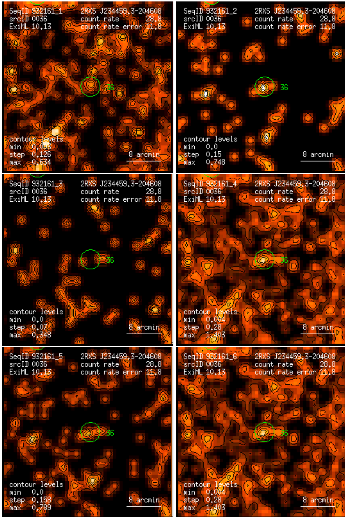
Figure 36: RASS 932161: detection 0036: band rate images, Gaussian filter: (1) PSPC channels 11 – 41, (2) 52 – 90, (3) 91 – 201, (4) 11 – 235, (5) 52 – 201, (6) 11 – 201. Broad band rates in counts/ks. Band rate contour levels in counts/ks/arcmin 2 .
