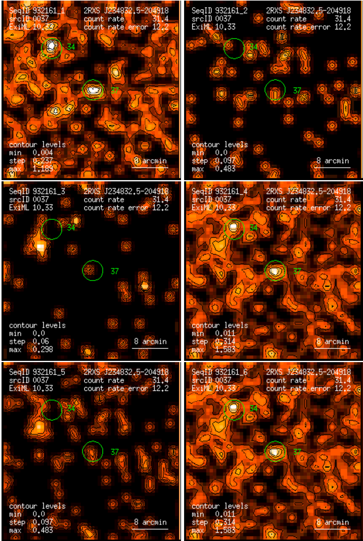
Figure 37: RASS 932161: detection 0037: band rate images, Gaussian filter: (1) PSPC channels 11 – 41, (2) 52 – 90, (3) 91 – 201, (4) 11 – 235, (5) 52 – 201, (6) 11 – 201. Broad band rates in counts/ks. Band rate contour levels in counts/ks/arcmin 2 .
