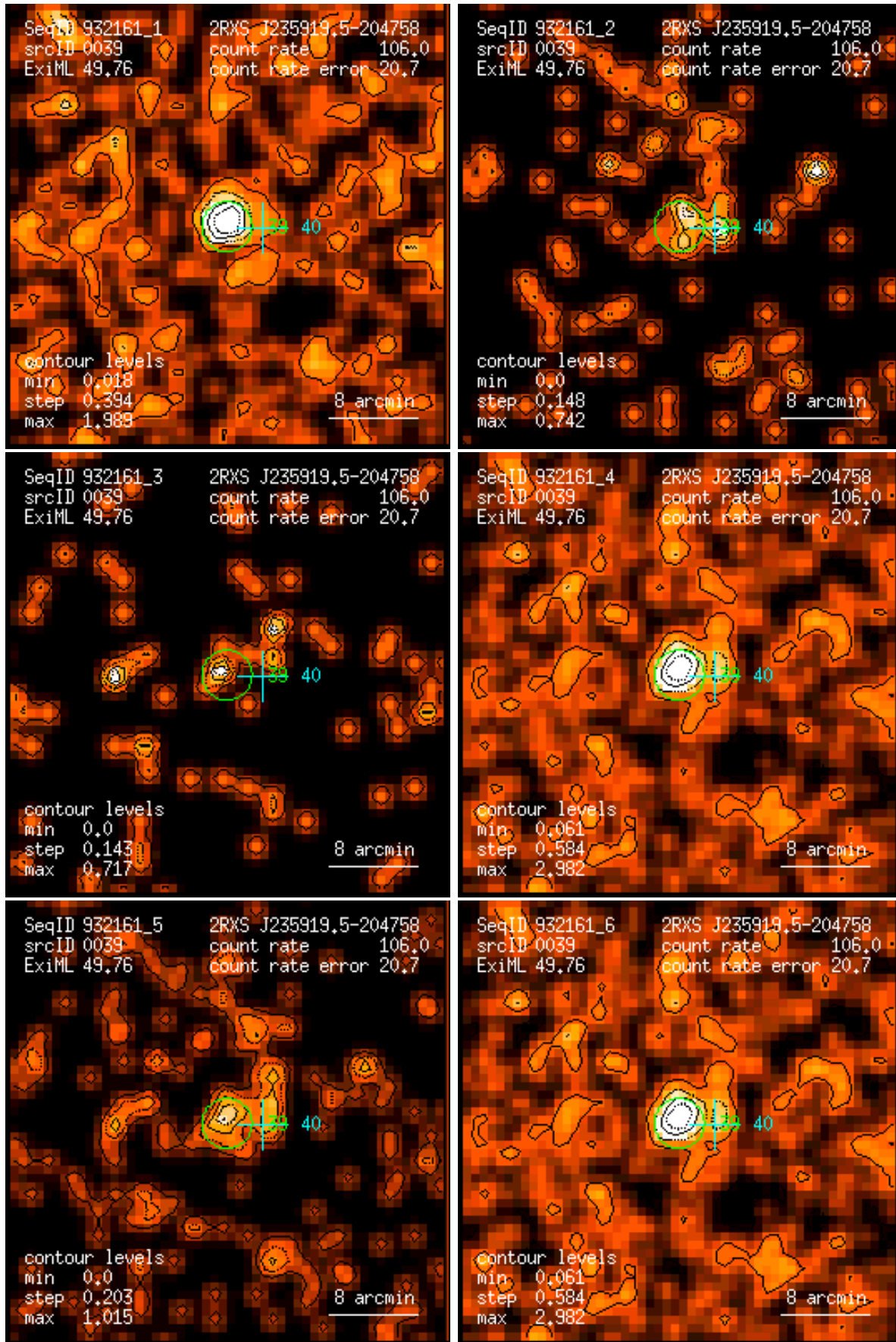
Figure 39: RASS 932161: detection 0039: band rate images, Gaussian filter: (1) PSPC channels 11 – 41, (2) 52 – 90, (3) 91 – 201, (4) 11 – 235, (5) 52 – 201, (6) 11 – 201. Broad band rates in counts/ks. Band rate contour levels in counts/ks/arcmin 2 .
