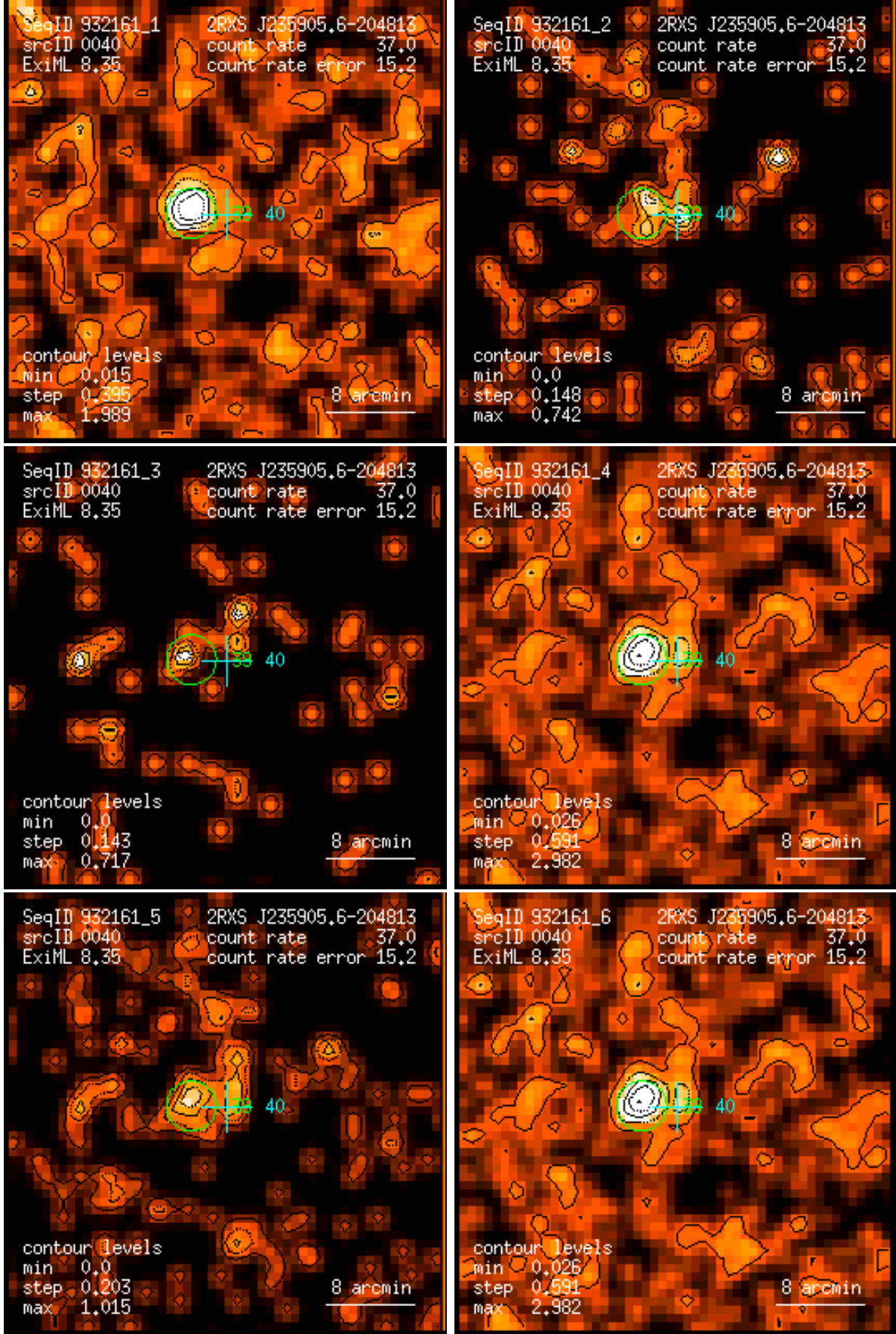
Figure 40: RASS 932161: detection 0040: band rate images, Gaussian filter: (1) PSPC channels 11 – 41, (2) 52 – 90, (3) 91 – 201, (4) 11 – 235, (5) 52 – 201, (6) 11 – 201. Broad band rates in counts/ks. Band rate contour levels in counts/ks/arcmin 2 .
