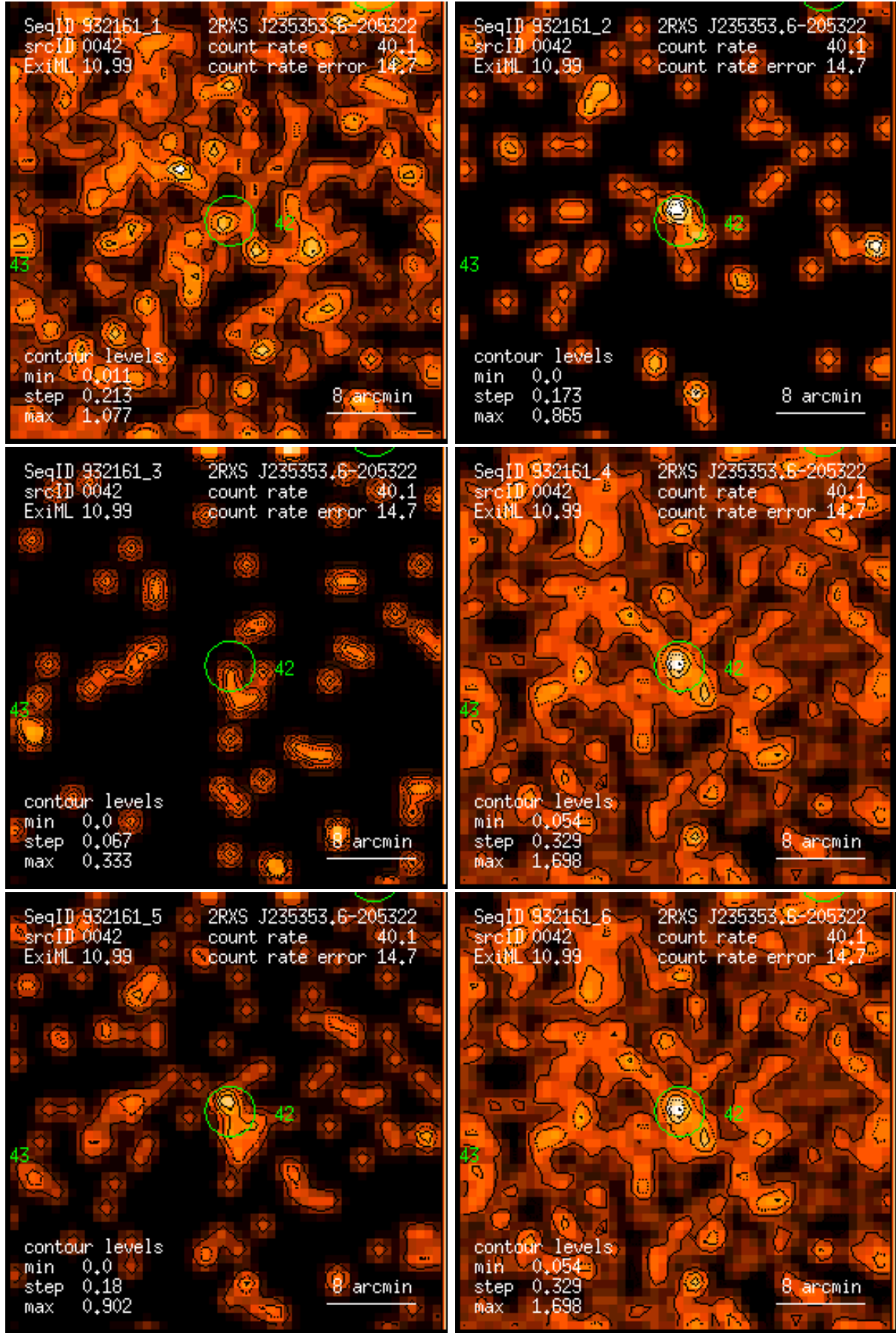
Figure 42: RASS 932161: detection 0042: band rate images, Gaussian filter: (1) PSPC channels 11 – 41, (2) 52 – 90, (3) 91 – 201, (4) 11 – 235, (5) 52 – 201, (6) 11 – 201. Broad band rates in counts/ks. Band rate contour levels in counts/ks/arcmin 2 .
