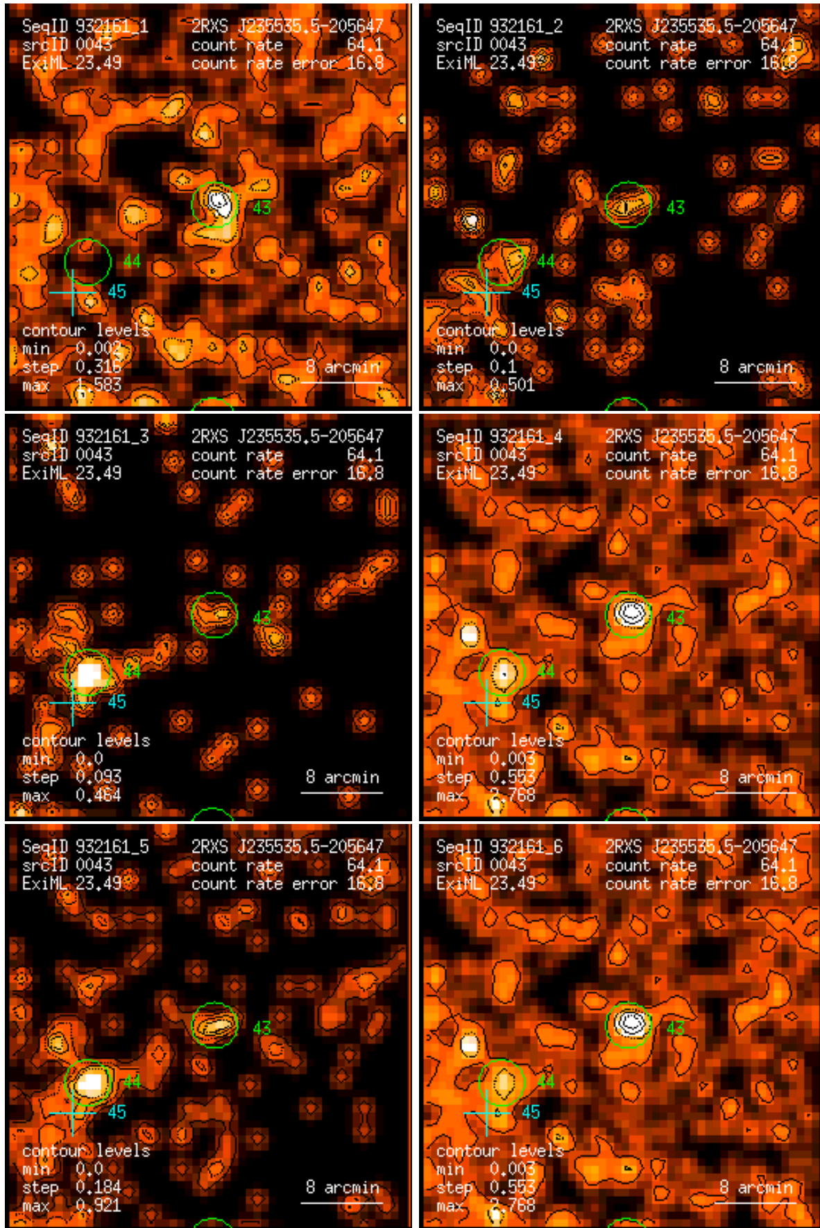
Figure 43: RASS 932161: detection 0043: band rate images, Gaussian filter: (1) PSPC channels 11 – 41, (2) 52 – 90, (3) 91 – 201, (4) 11 – 235, (5) 52 – 201, (6) 11 – 201. Broad band rates in counts/ks. Band rate contour levels in counts/ks/arcmin 2 .
