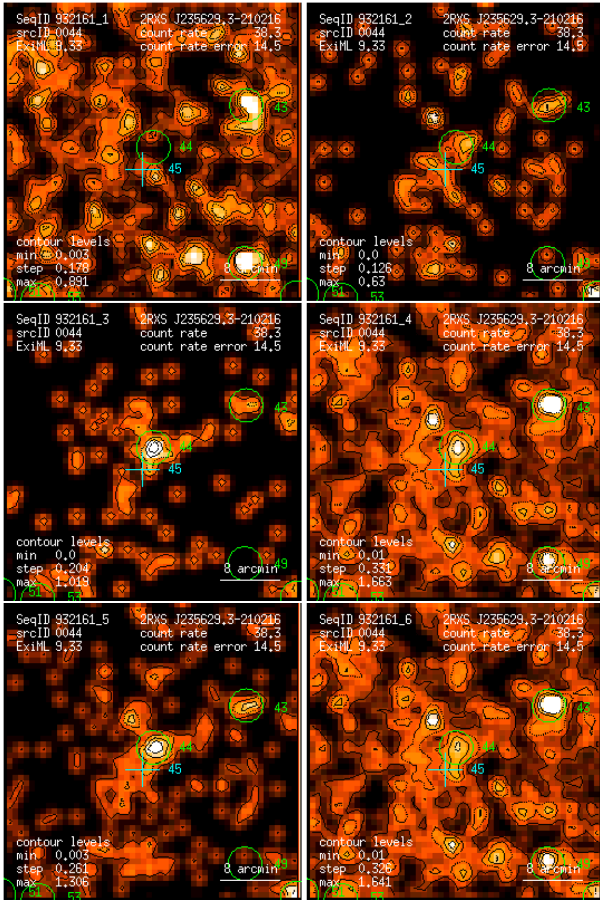
Figure 44: RASS 932161: detection 0044: band rate images, Gaussian filter: (1) PSPC channels 11 – 41, (2) 52 – 90, (3) 91 – 201, (4) 11 – 235, (5) 52 – 201, (6) 11 – 201. Broad band rates in counts/ks. Band rate contour levels in counts/ks/arcmin 2 .
