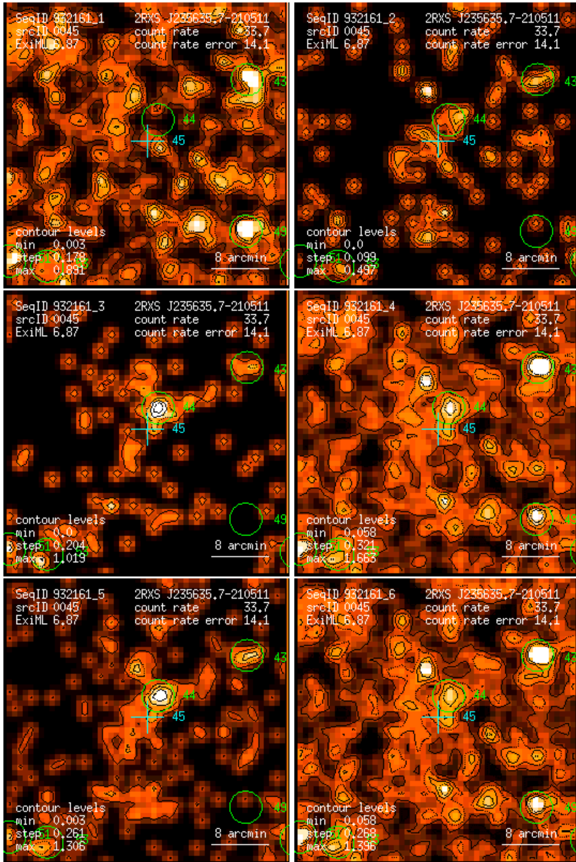
Figure 45: RASS 932161: detection 0045: band rate images, Gaussian filter: (1) PSPC channels 11 – 41, (2) 52 – 90, (3) 91 – 201, (4) 11 – 235, (5) 52 – 201, (6) 11 – 201. Broad band rates in counts/ks. Band rate contour levels in counts/ks/arcmin 2 .
