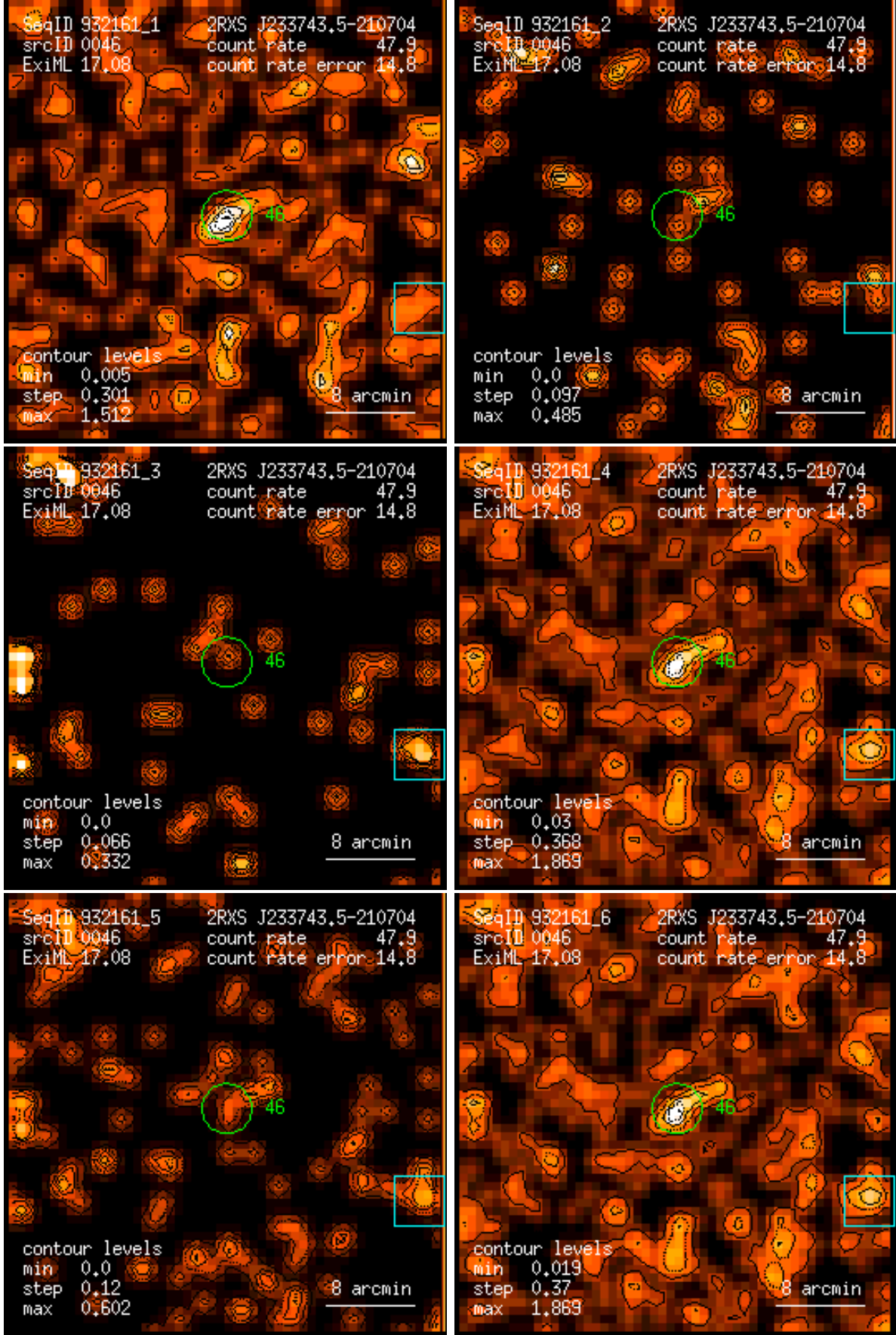
Figure 46: RASS 932161: detection 0046: band rate images, Gaussian filter: (1) PSPC channels 11 – 41, (2) 52 – 90, (3) 91 – 201, (4) 11 – 235, (5) 52 – 201, (6) 11 – 201. Broad band rates in counts/ks. Band rate contour levels in counts/ks/arcmin 2 .
