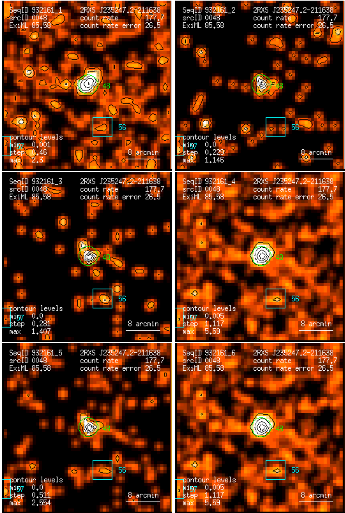
Figure 48: RASS 932161: detection 0048: band rate images, Gaussian filter: (1) PSPC channels 11 – 41, (2) 52 – 90, (3) 91 – 201, (4) 11 – 235, (5) 52 – 201, (6) 11 – 201. Broad band rates in counts/ks. Band rate contour levels in counts/ks/arcmin 2 .
