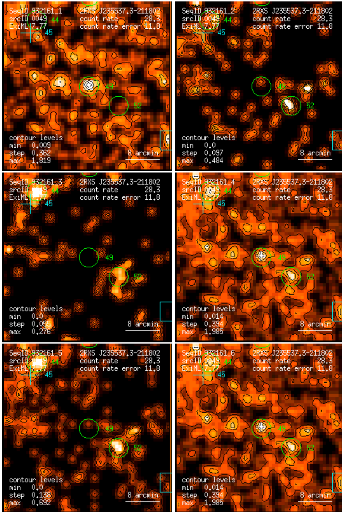
Figure 49: RASS 932161: detection 0049: band rate images, Gaussian filter: (1) PSPC channels 11 – 41, (2) 52 – 90, (3) 91 – 201, (4) 11 – 235, (5) 52 – 201, (6) 11 – 201. Broad band rates in counts/ks. Band rate contour levels in counts/ks/arcmin 2 .
