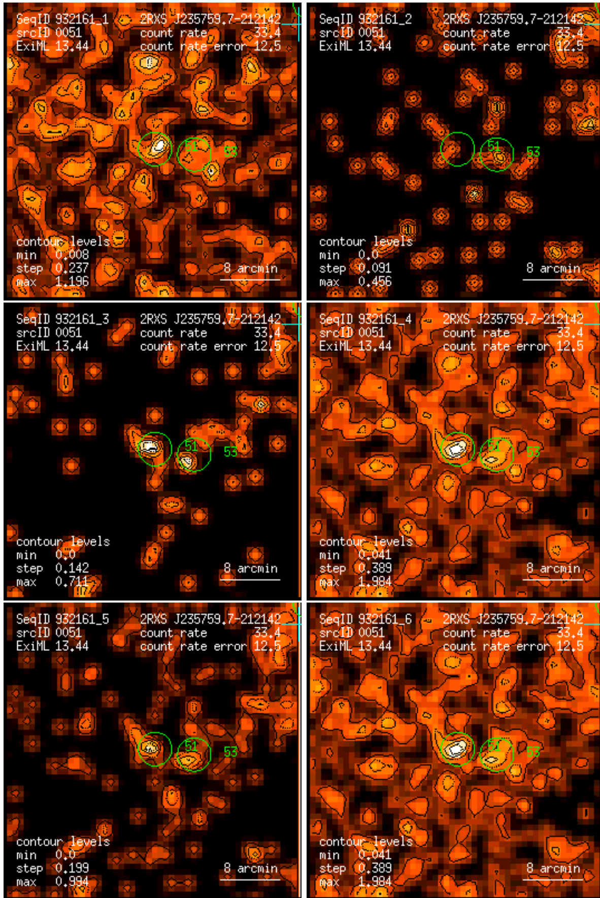
Figure 51: RASS 932161: detection 0051: band rate images, Gaussian filter: (1) PSPC channels 11 – 41, (2) 52 – 90, (3) 91 – 201, (4) 11 – 235, (5) 52 – 201, (6) 11 – 201. Broad band rates in counts/ks. Band rate contour levels in counts/ks/arcmin 2 .
