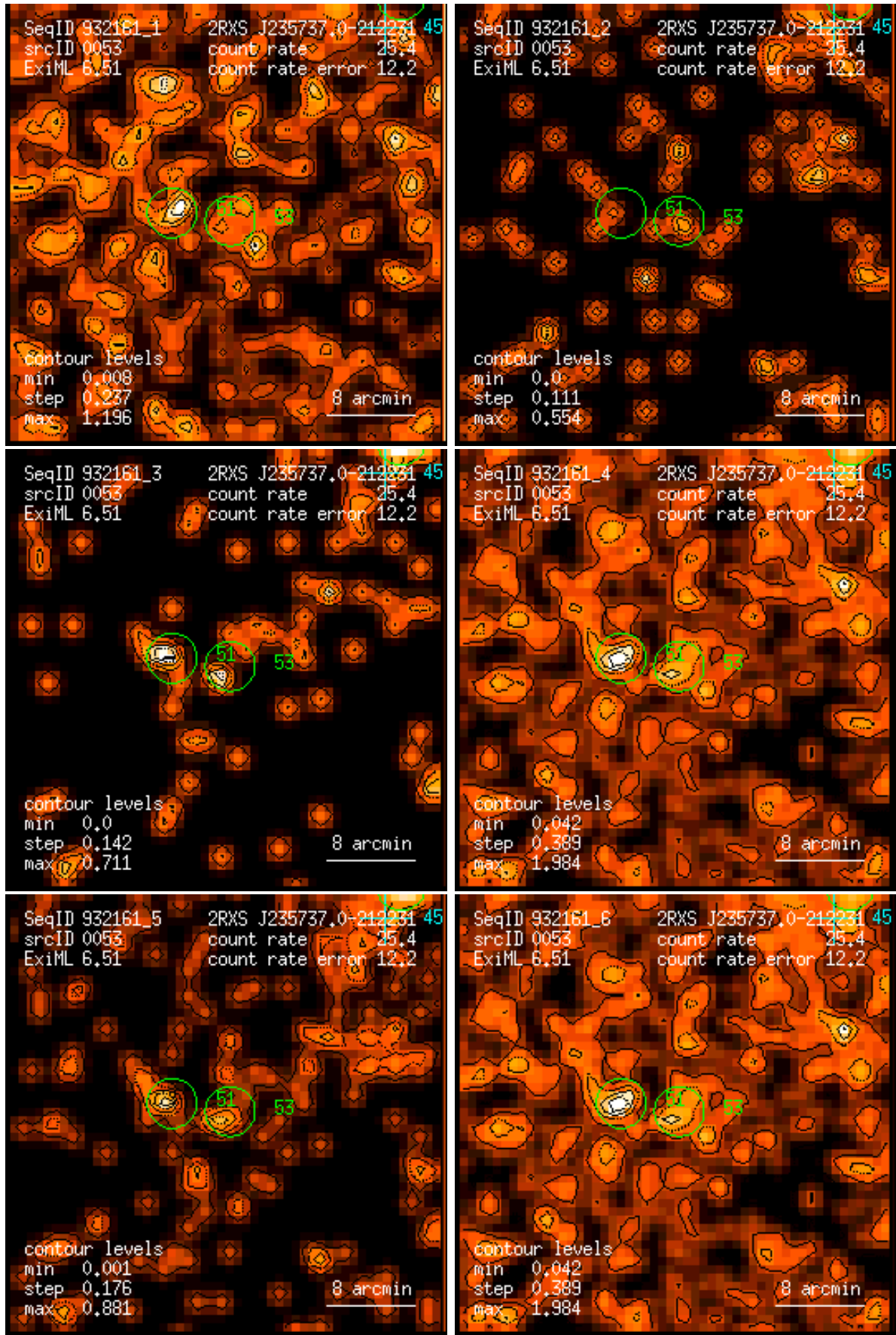
Figure 53: RASS 932161: detection 0053: band rate images, Gaussian filter: (1) PSPC channels 11 – 41, (2) 52 – 90, (3) 91 – 201, (4) 11 – 235, (5) 52 – 201, (6) 11 – 201. Broad band rates in counts/ks. Band rate contour levels in counts/ks/arcmin 2 .
